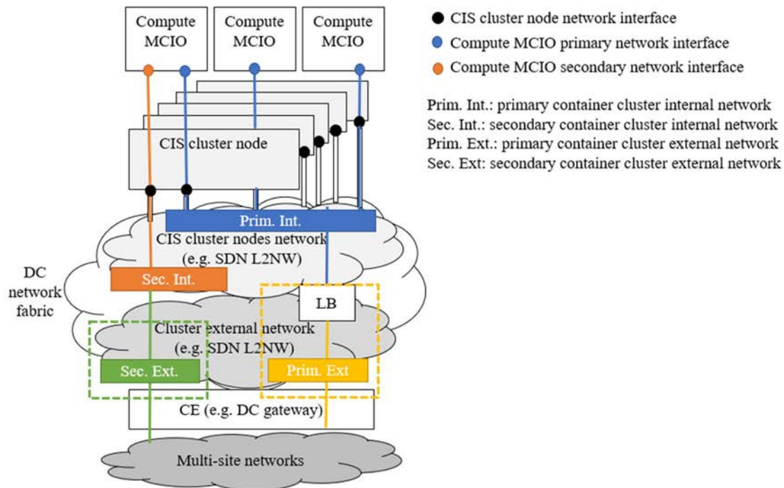
Figure 4.2.6.3-1: Types of container cluster network on setup on CIS cluster
