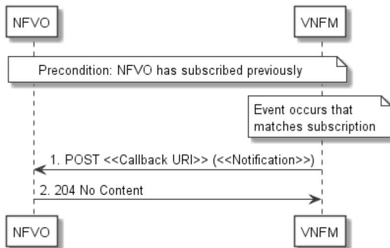
Figure 5.3.9-1: Flow of sending notifications
