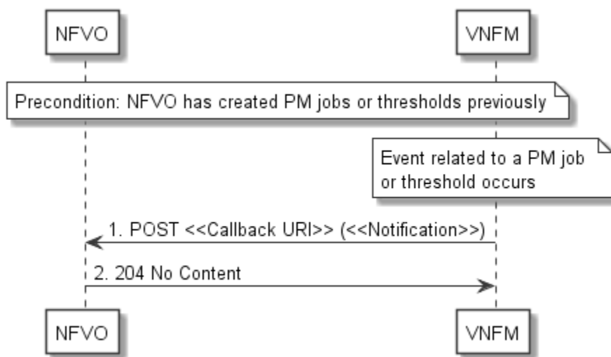
Figure 6.3.9-1: Flow of sending notifications
