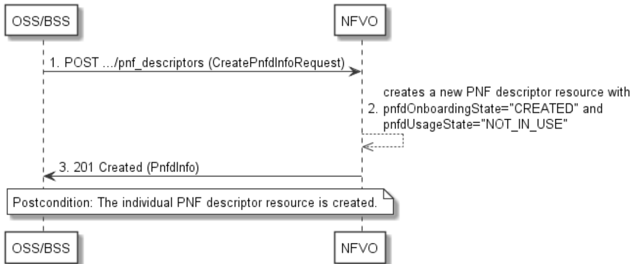
Figure 5.3.7-1: Flow of the creation of an individual PNF descriptor resource
