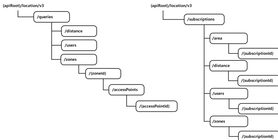
Figure 7.2-1: Resource URI structure of the Location API
