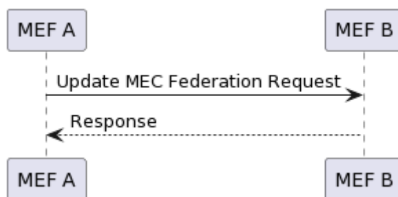
Figure 5.2.4.3-1: Information flow of Update
