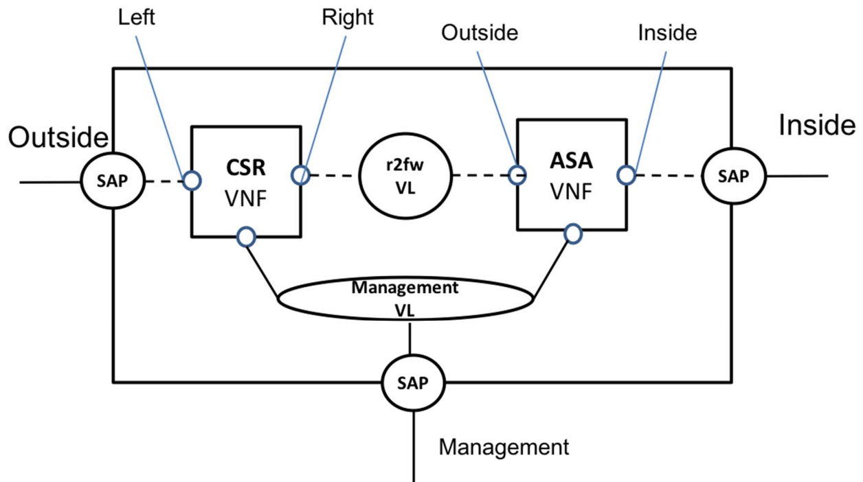
Figure A.2-1: Firewall Router Example
