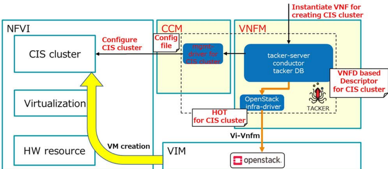
Figure A.5.4.3-1: Creation of VM based CIS cluster by OpenStack® Tacker
