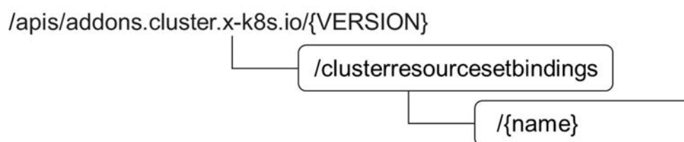
Figure 7.3-2: Resource URI structure of ClusterResourceSetBinding resource object for the CIS cluster configuration management service interface
