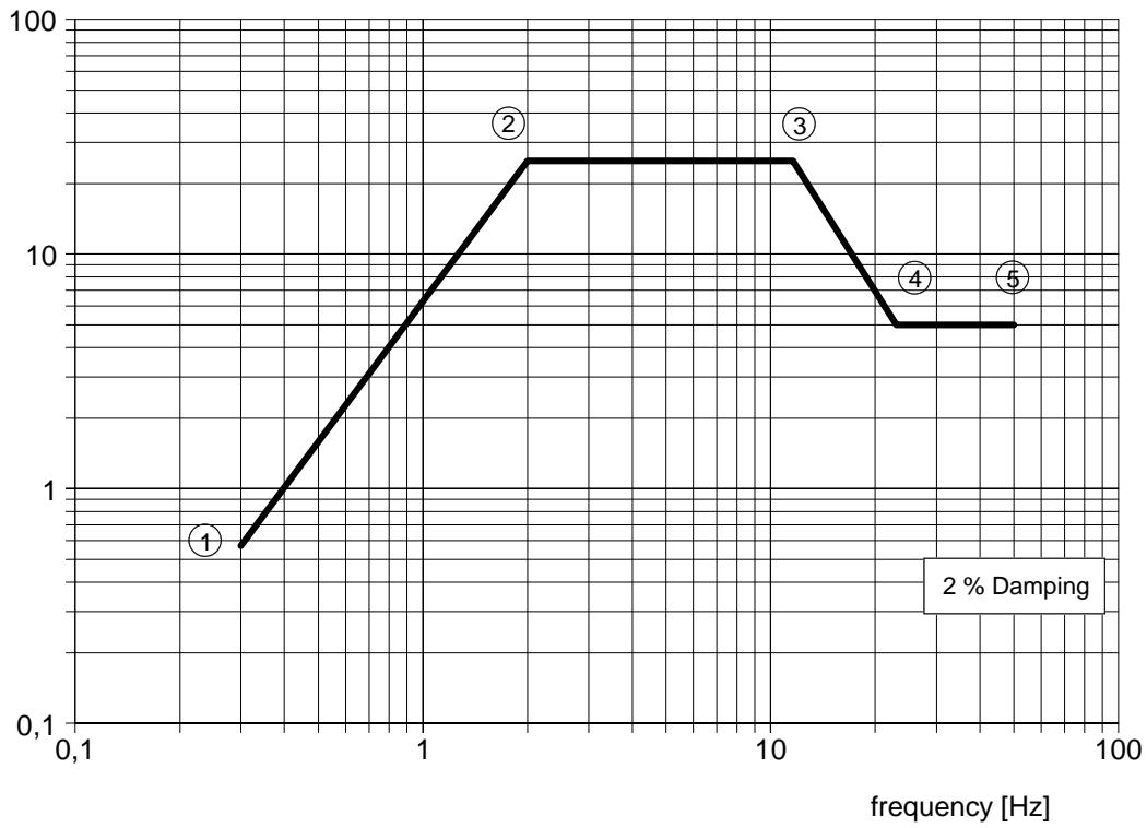
Figure 3: Earthquake Response Spectrum
