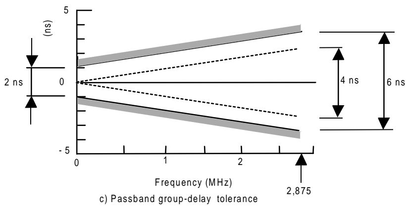
Figure F.1: Specification for a luminance or RGB signal filter used when sampling at 6,75 MHz
