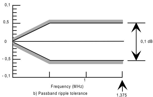
Figure F.3: Specification for a digital filter for sampling-rate conversion from 2:2:2 to 2:1:1 colour-difference-signals
