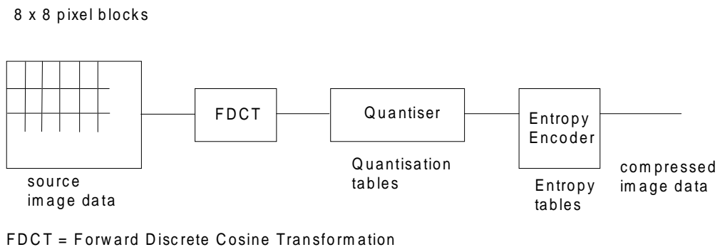
Figure A.5: DCT-based encoder functional blocks
