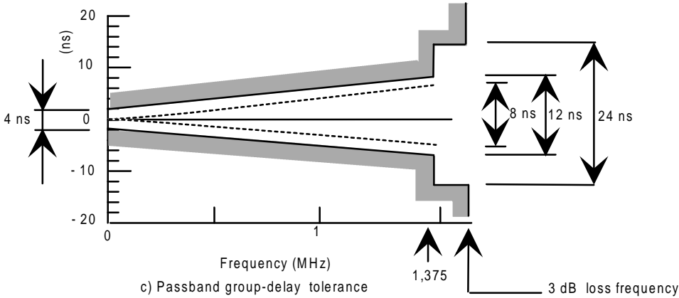
Figure F.2: Specification for a colour-difference signal filter used when sampling at 3,375 MHz
