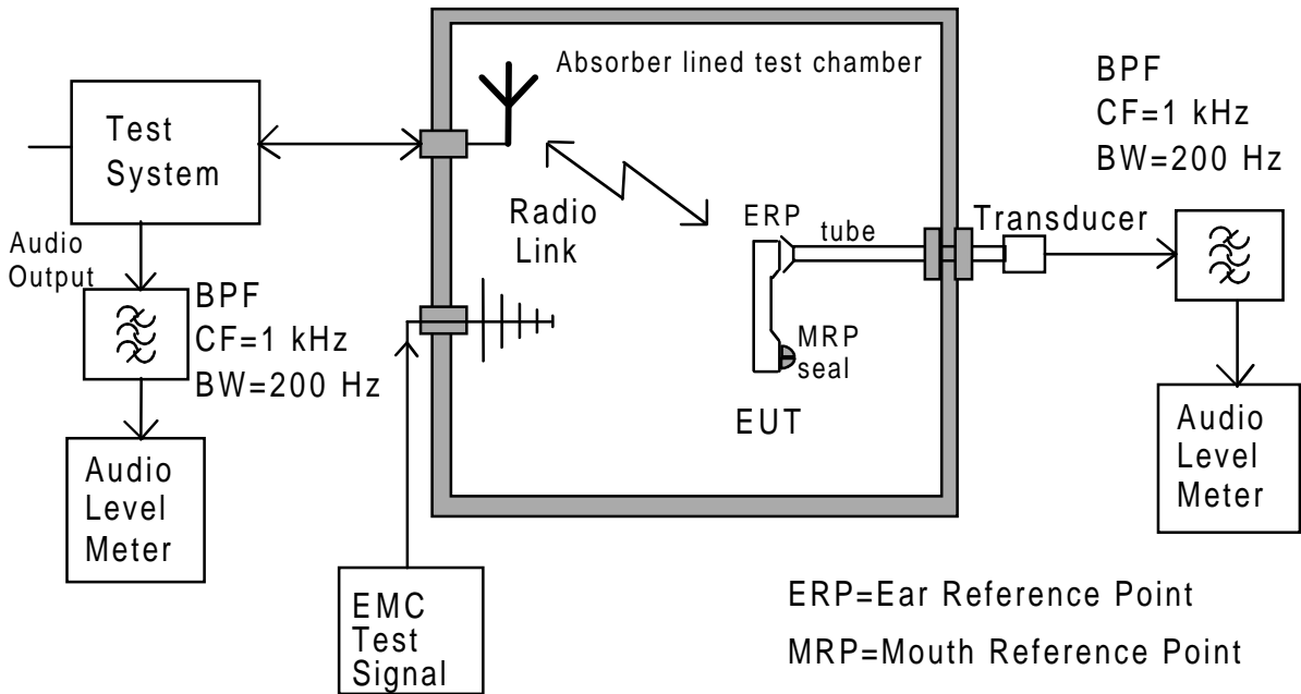
Figure 1: Audio breakthrough measurement, test set-up
