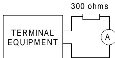
Figure A.9: Power feeding
