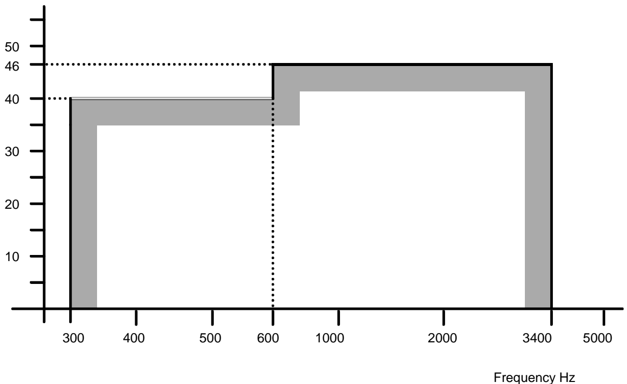
Figure 1: Longitudinal conversion loss, minimum values
