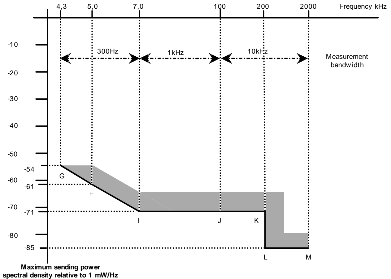
Figure 3: Maximum sending power outside the voice bandwidth (spectral density)
