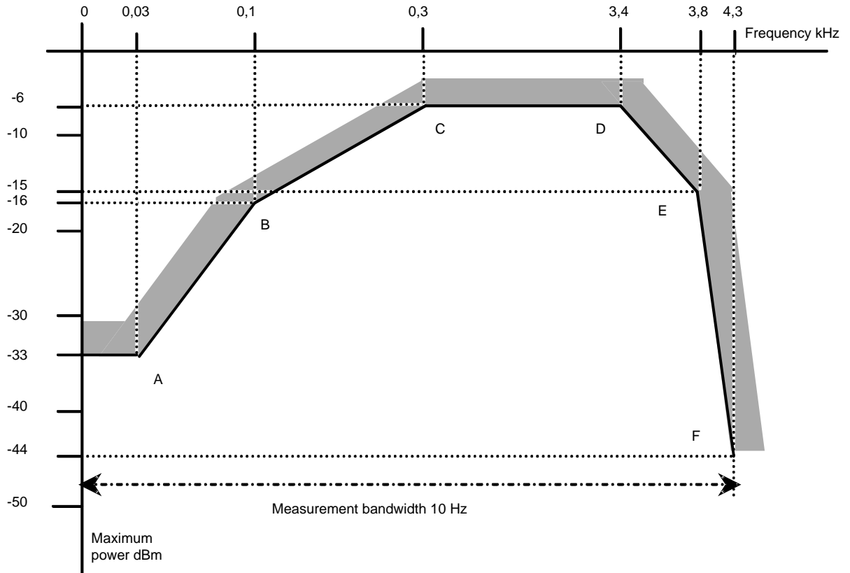
Figure 2: Maximum power in a 10 Hz bandwidth
