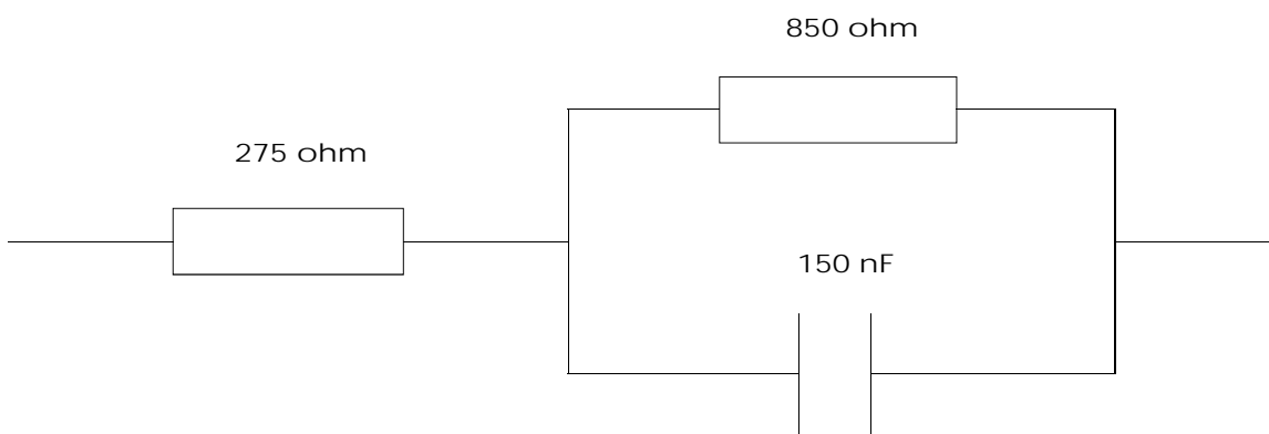
Figure A.1: Reference impedance
