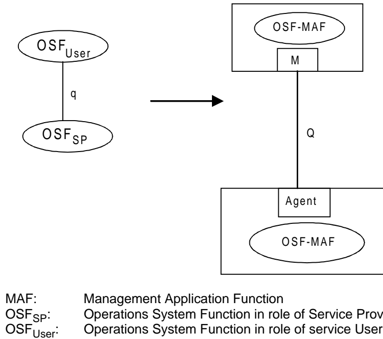
Figure 1: Service provider and service user roles of OSFs
