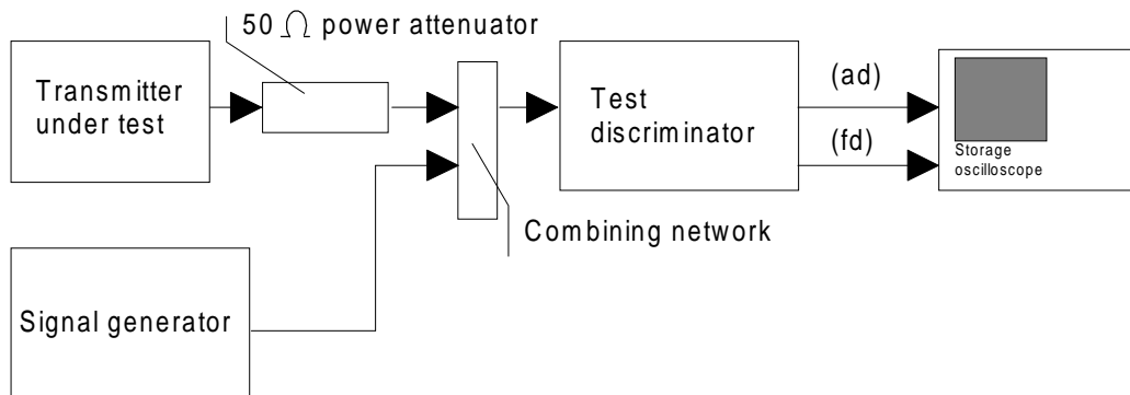
Figure 3: Measurement arrangement
