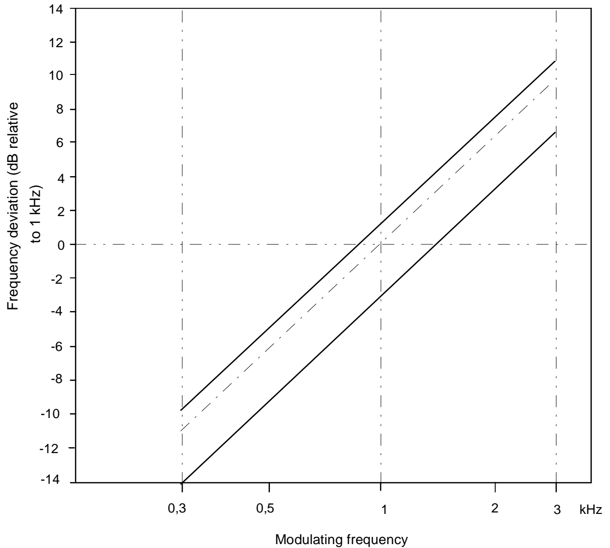
Figure 2: Audio frequency response
