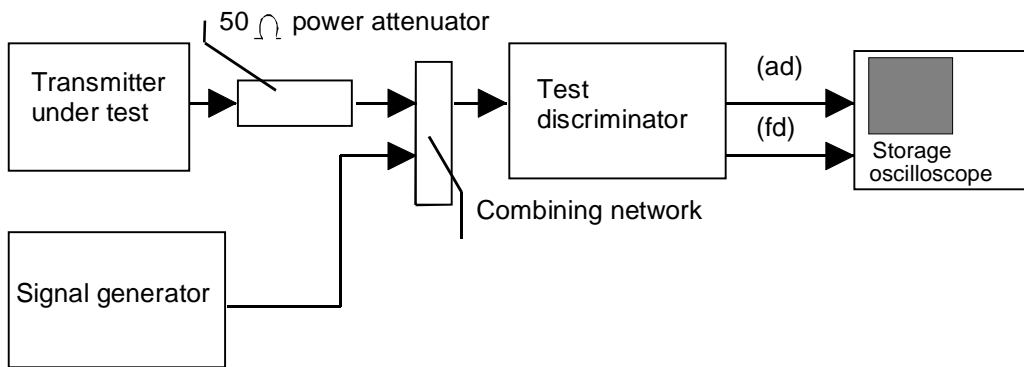
Figure 3: Measurement arrangement
