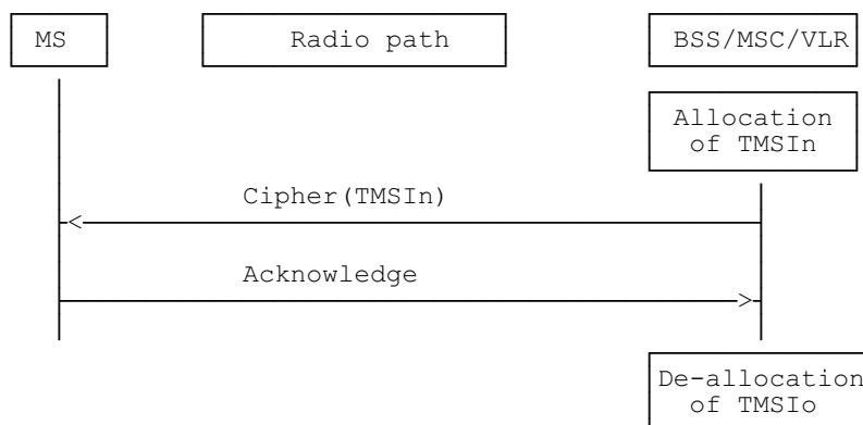
Figure 2.5: Reallocation of a new TMSI
