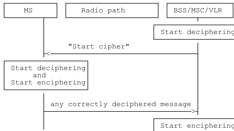
Figure 4.2: Starting of the encipherng and deciphering processes
