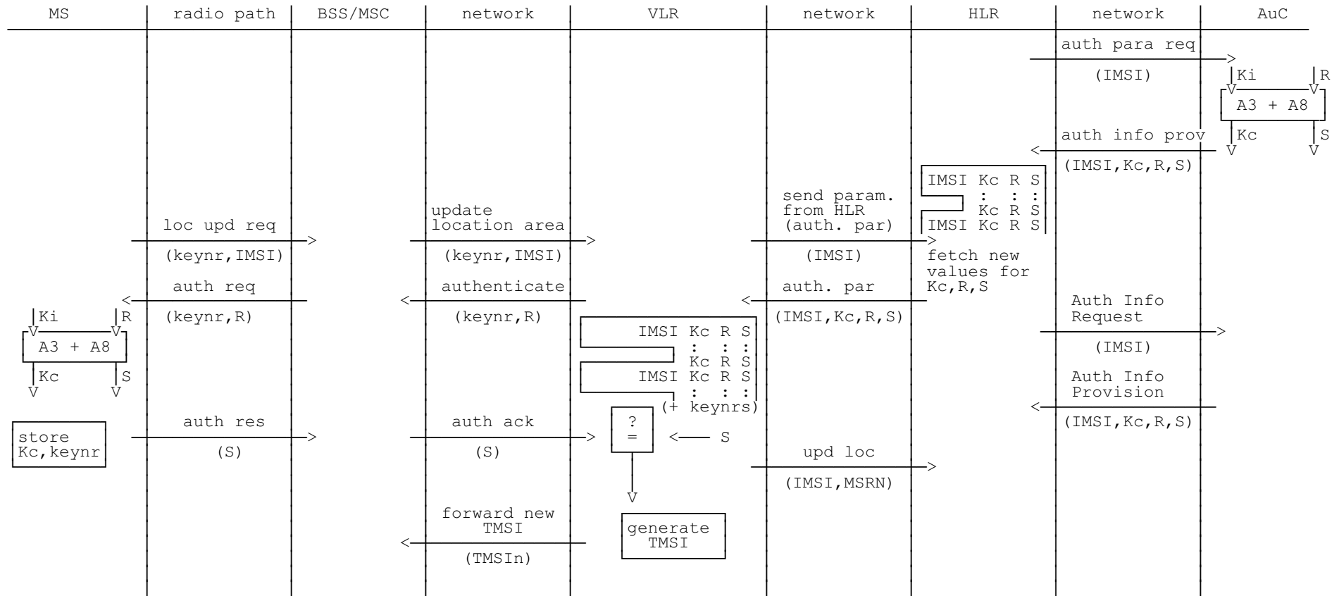
Scheme 1 Location registration - no TMSI available
