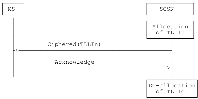
Figure D.2.4: Reallocation of a new TLLI
