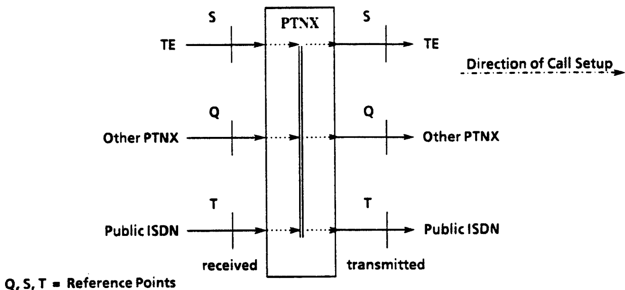
Figure 39 - Numbering Formats for Selection Numbers
