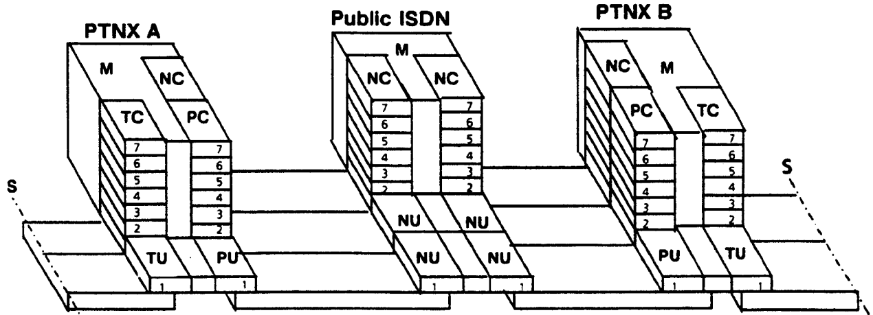
Figure 30 - Protocol Model for the Circuit-Switched Link Scenario
