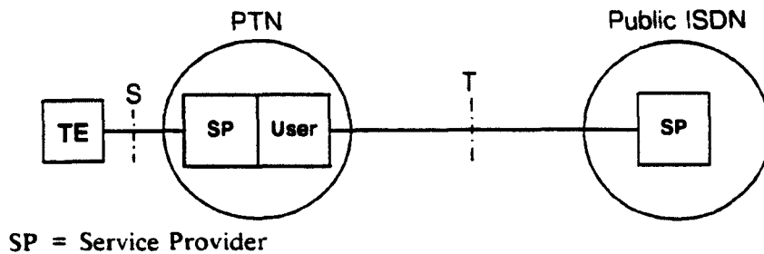
Figure 46 - Example of Dual Provision of a Supplementary Service
