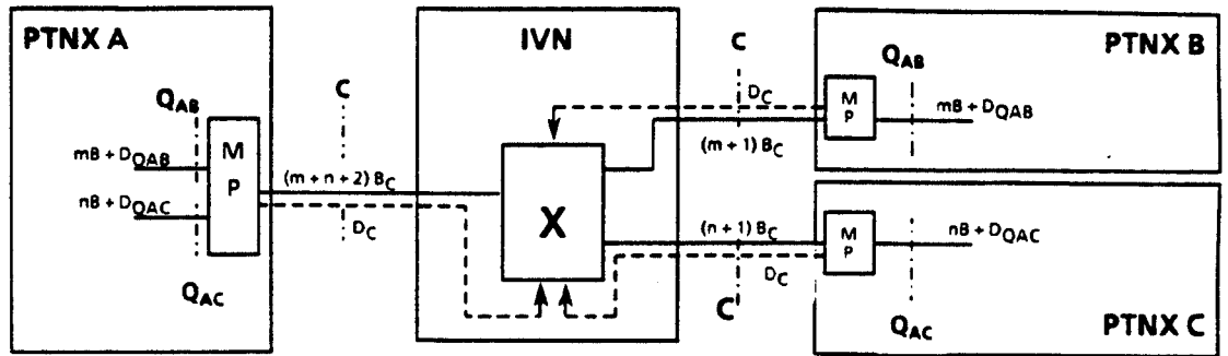
Figure 22 - On-Demand Circuit-Switched
