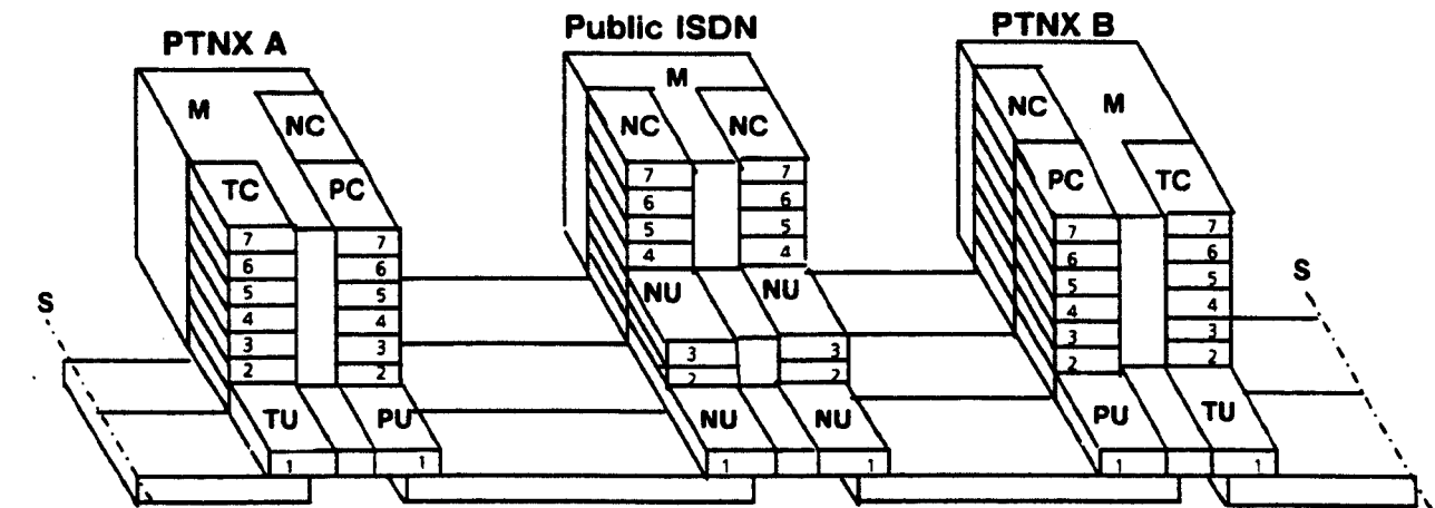
Figure 32 - Protocol Model for On-Demand Virtual Call
