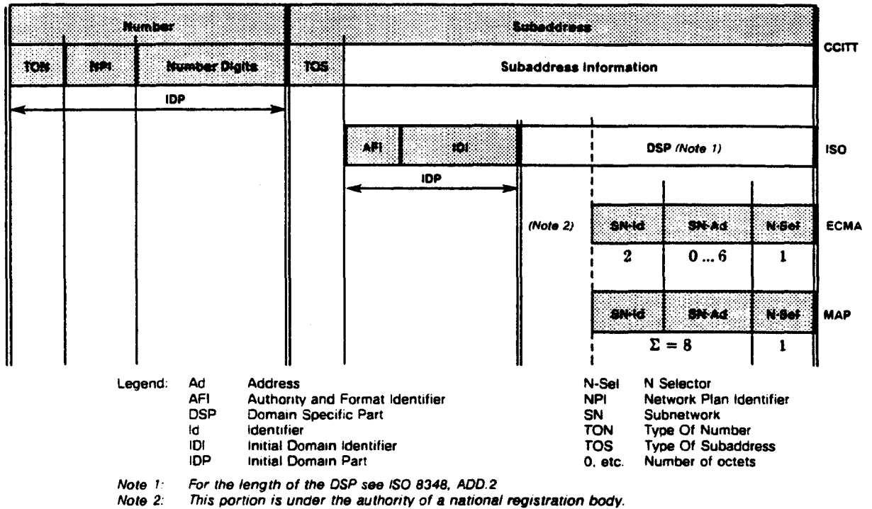
Figure 37 - Addressing Principles
