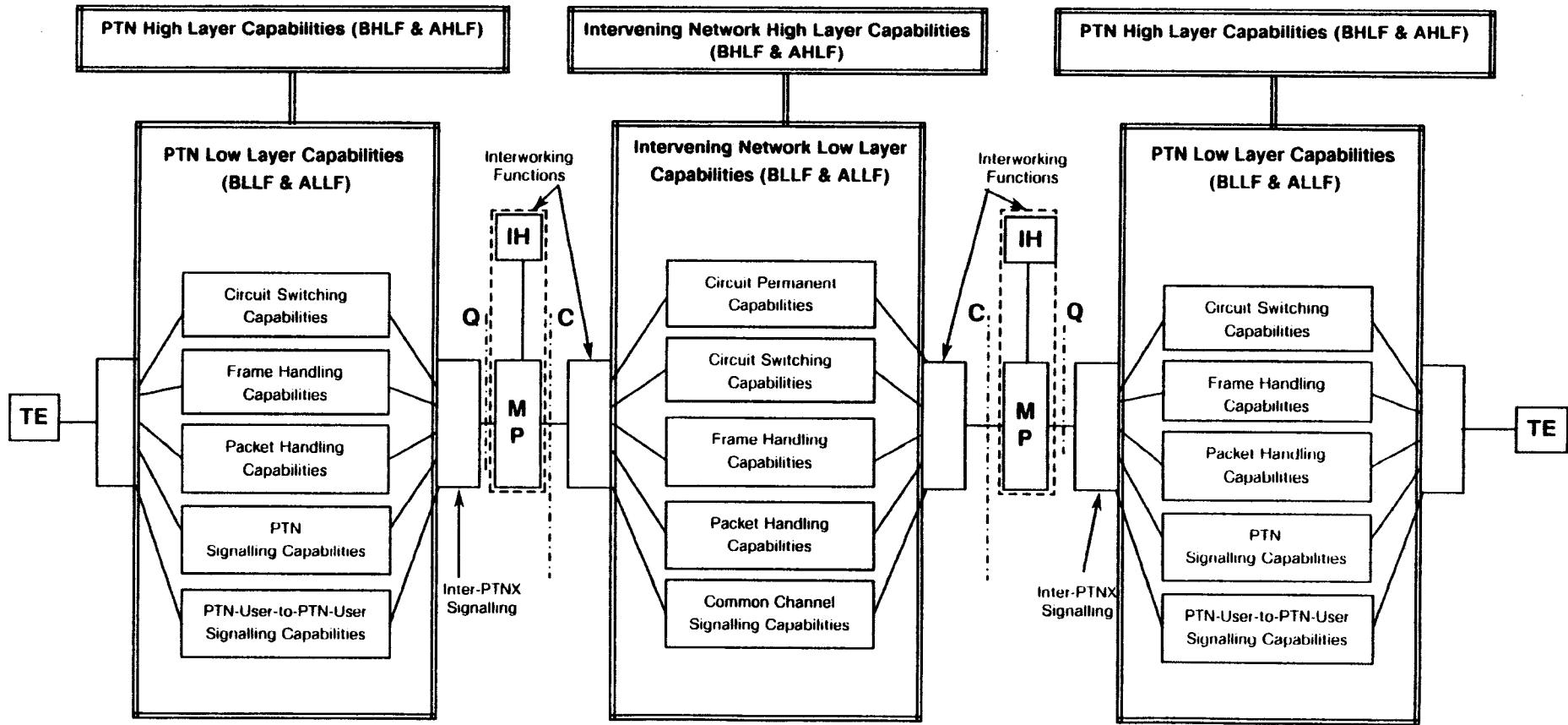
Figure 13 - Overall Architecture of a Private Telecommunication Network Employing a Public ISDN as an Intervening Network
