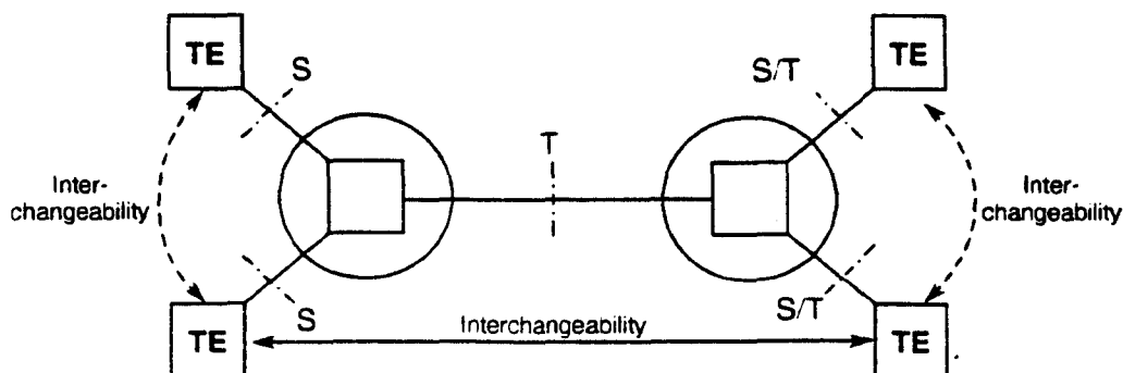
Figure 43 - Terminal Interchangeability
