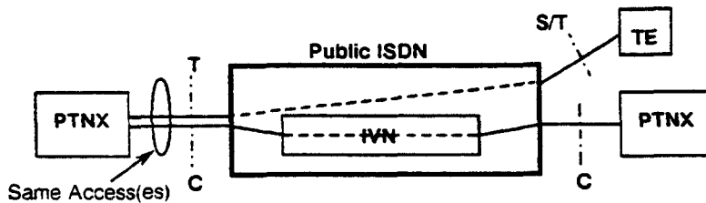
Figure 16 - Shared Access Use
