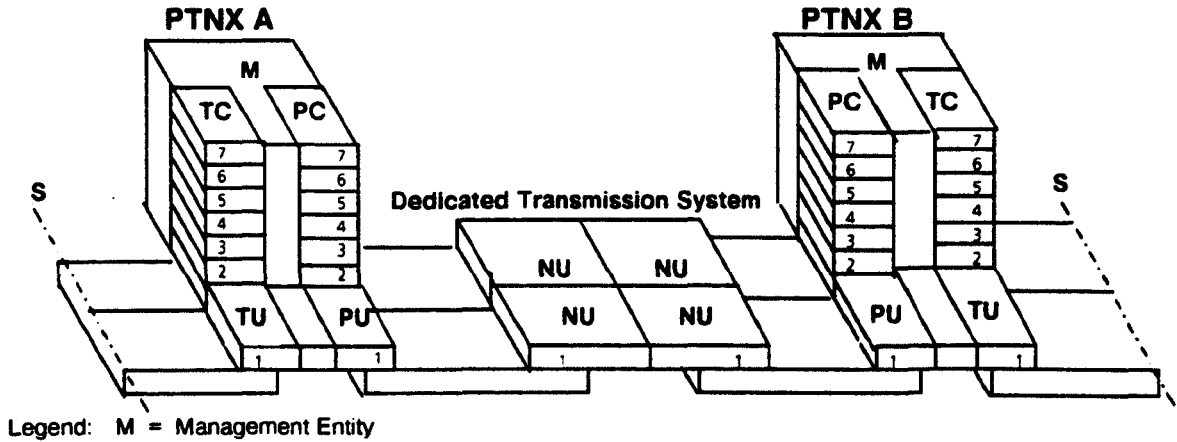
Figure 26 - Protocol Model for the Dedicated Transmission System Scenario
