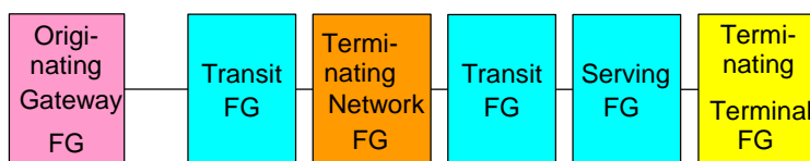
Figure A.15: TIPHON Scenario 2 - terminating user roaming
