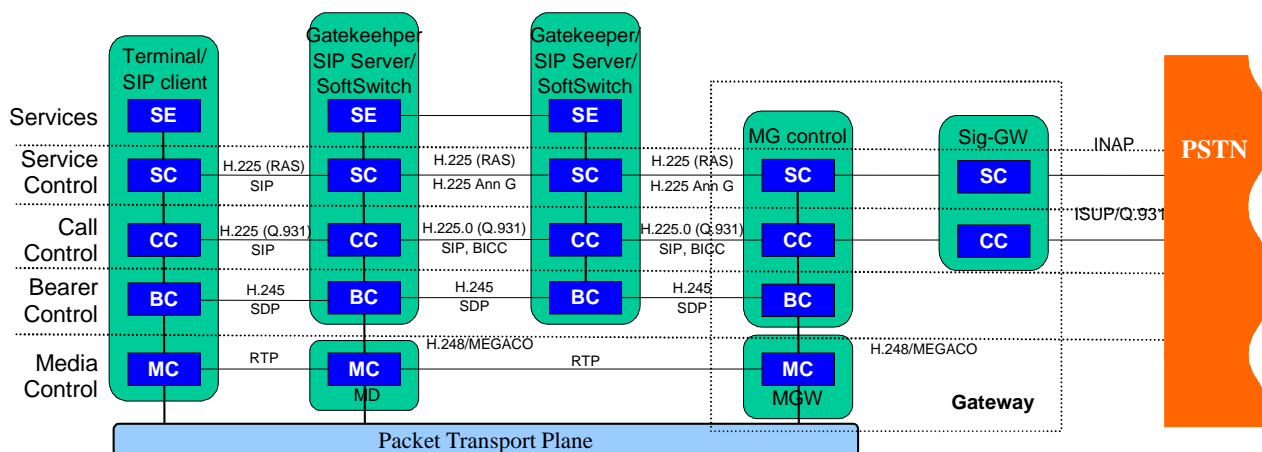
Figure A.24: Mapping to physical entities and protocols
