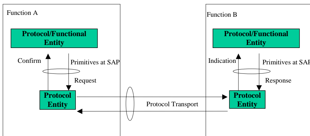
Figure A.20: Relationship of functional entities, primitives and protocols
