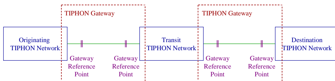
Figure 9: Simple TIPHON reference model
