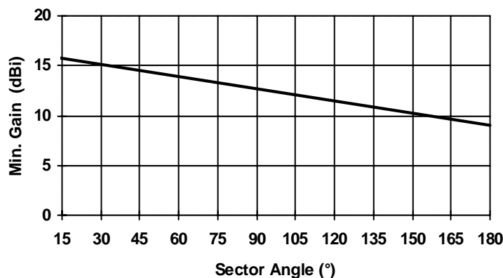
Figure 4: CS sector antenna minimum boresight gain limits
