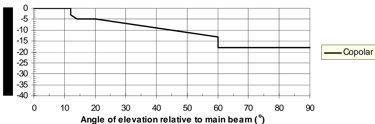
Figure 5: Symmetric CS antenna elevation pattern, range 1
