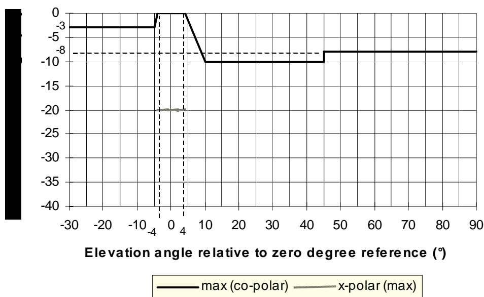
Figure 7: Asymmetric CS antenna elevation patterns
