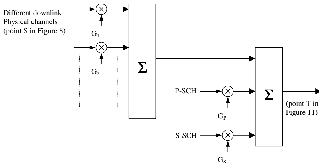
Figure 5.19: Downlink channels combination and Spreading for SCH
