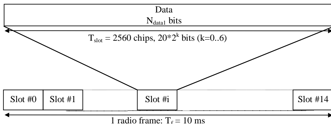
Figure 5.13: Frame structure of PDSCH
