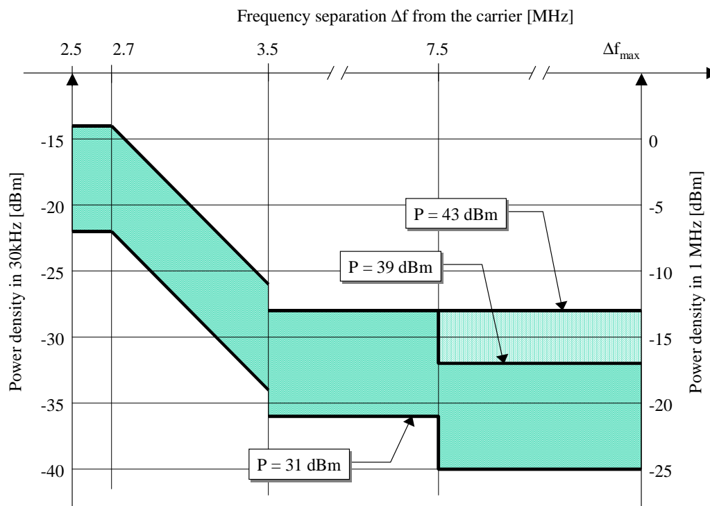
Illustrative diagram of spectrum emission mask
