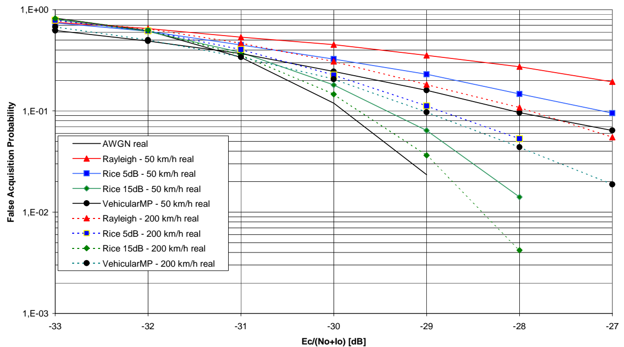
Figure 6.20: False Acquisition probability vs. E_c/N_o , step 2
