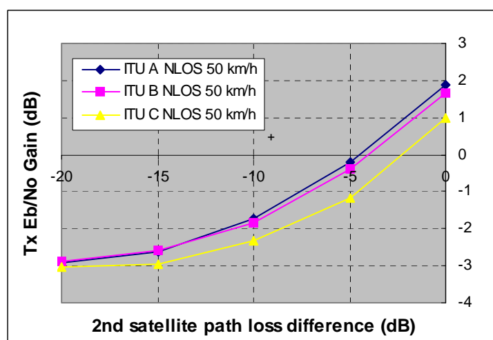
Figure 6.10: Satellite diversity gain; NLOS; Downlink; 50 km/h
