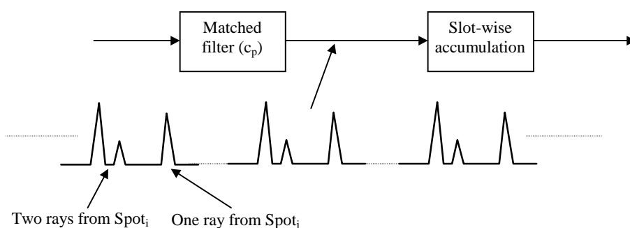
Figure 5.30: Matched-filter search for primary synchronization code
