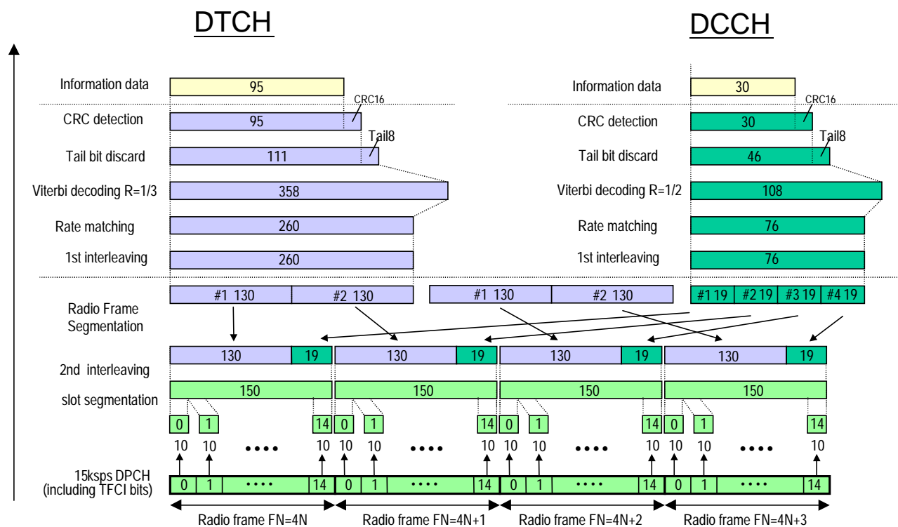
Figure B.1: Channel coding and multiplexing example for 4,75 kbps data; Uplink
