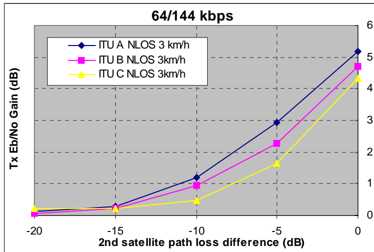
Figure 6.6: Satellite diversity gain; NLOS; Uplink; 64/144 kbps; 3 km/h
