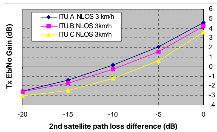
Figure 6.9: Satellite diversity gain; NLOS; Downlink; 3 km/h
