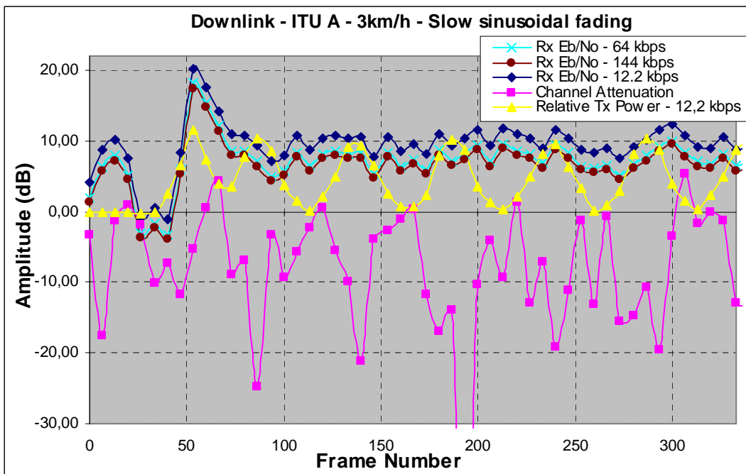
Figure 6.16: Slow Power Control Response to sinusoidal fading; ITU Model A; Downlink
