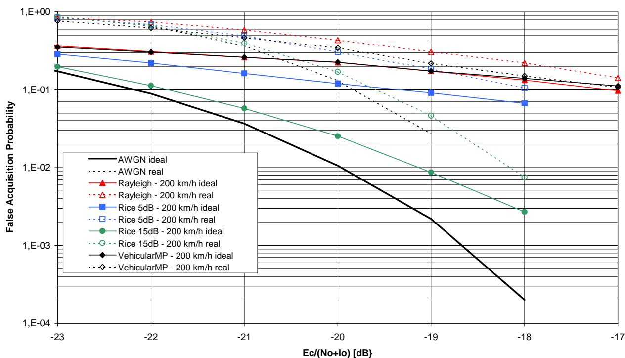
Figure 6.22: False Acquisition probability vs. E_c/N_o , step 3, 200 km/h
