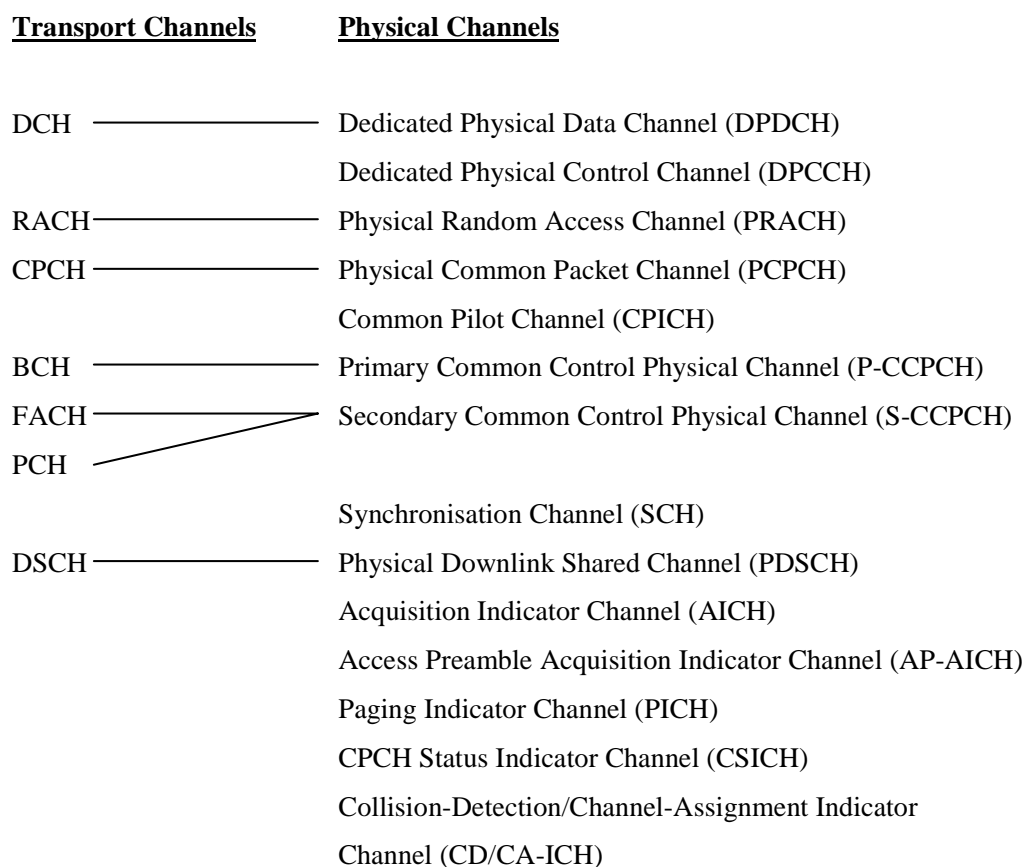
Figure 5.4: Mapping of Transport channels onto Physical channels
