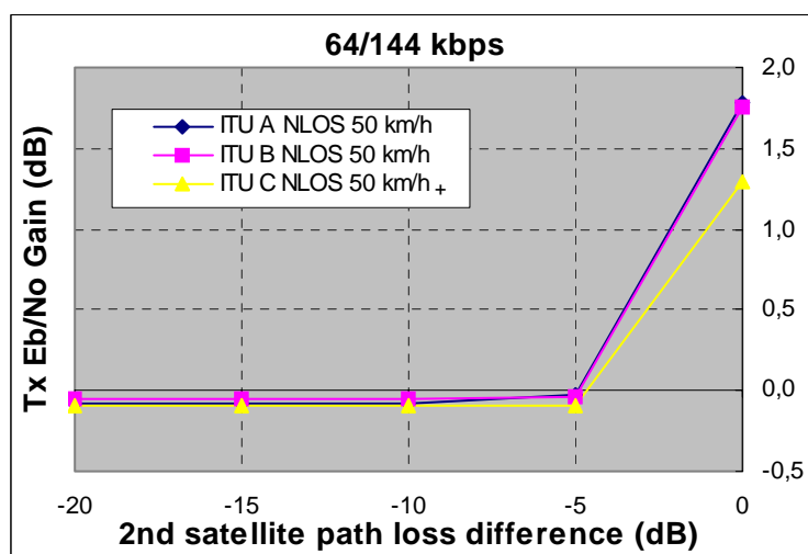
Figure 6.8: Satellite diversity gain; NLOS; Uplink; 64/144 kbps; 50 km/h
