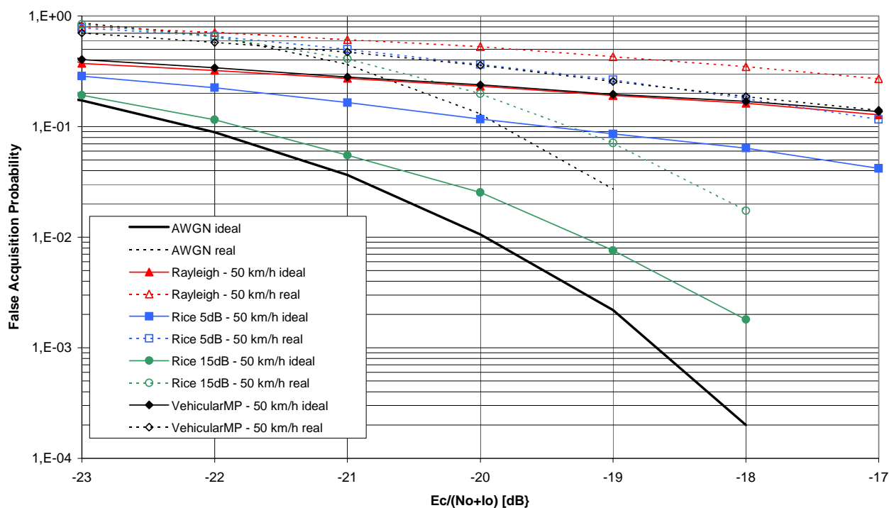
Figure 6.21: False Acquisition probability vs. E_c/N_o , step 3, 50 km/h
