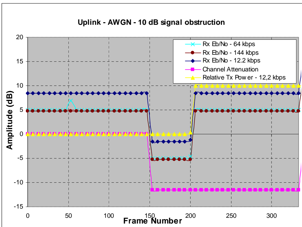
Figure 6.13: Slow Power Control Response to 10 dB Signal obstruction; AWGN; Uplink
