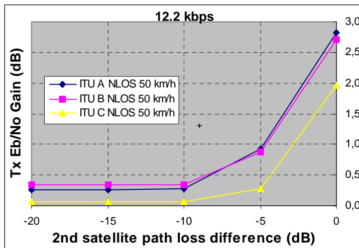
Figure 6.7: Satellite diversity gain; NLOS; Uplink; 12,2 kbps; 50 km/h
