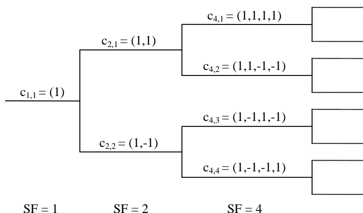
Figure 5.20: Code-tree for generation of OVFS codes
