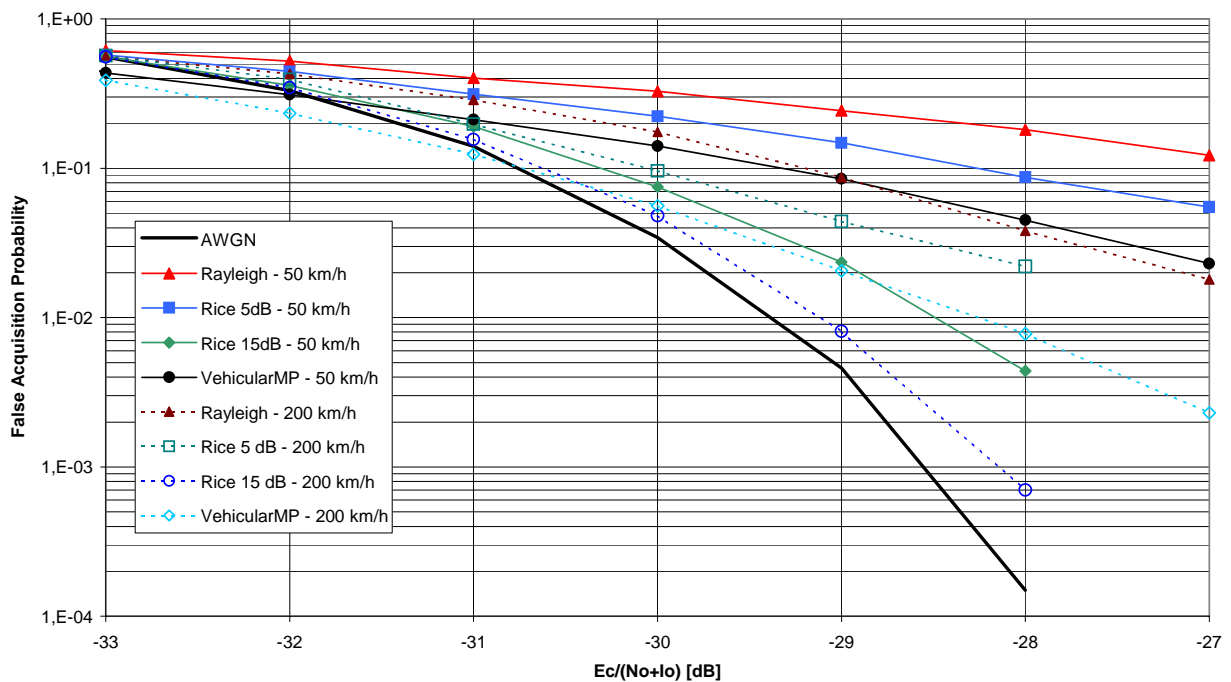
Figure 6.19: False Acquisition probability vs. E_c/N_o , step 1
