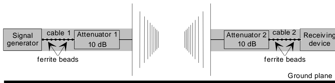
Figure 39: Stage 2: NSA measurement
