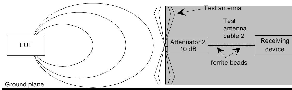
Figure 55: Stage 2: EUT measurement
