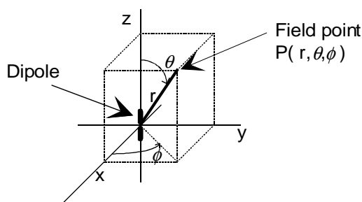
Figure 18: Spherical co-ordinates
