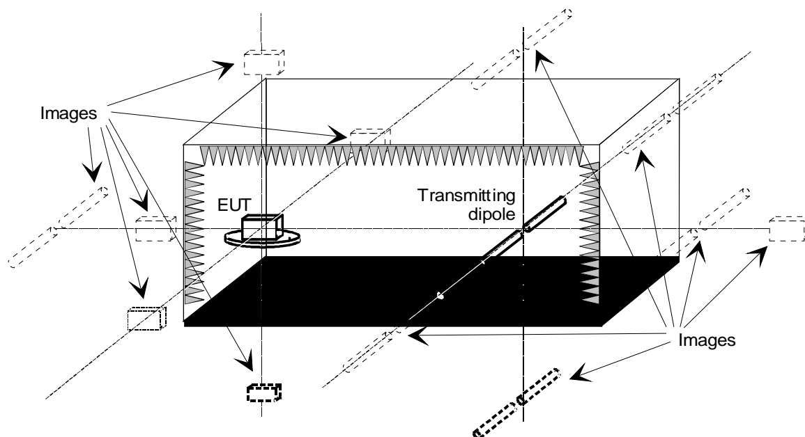
Figure 2: Imaging in the shielded enclosure
