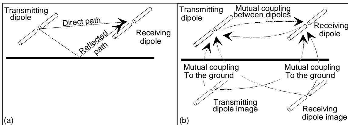
Figure 23: (a) Ideal model of a ground reflection site and (b) Mutual coupling effects on a real site
