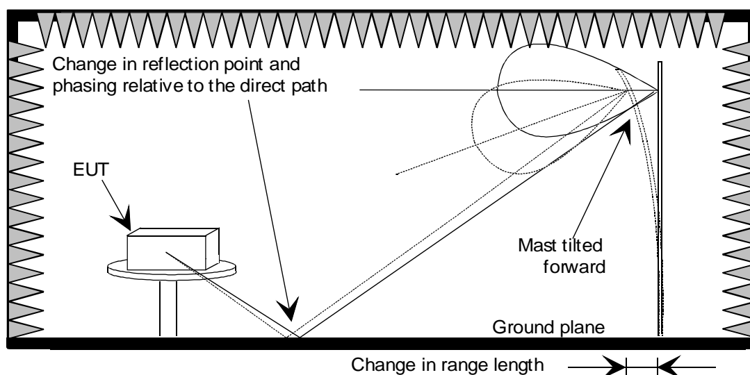
Figure 17: Mast stability
