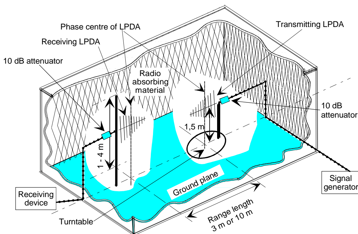
Figure 33: Anechoic Chamber with a Ground Plane layout for verification with LPDAs
