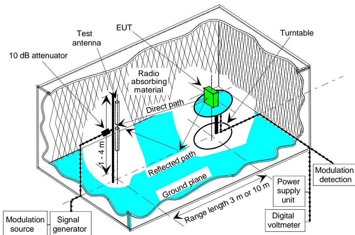
Figure 53: Anechoic Chamber with a Ground Plane set-up for Sensitivity tests on the EUT
