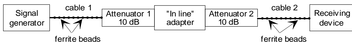
Figure 28: Initial equipment arrangement for the verification procedure
