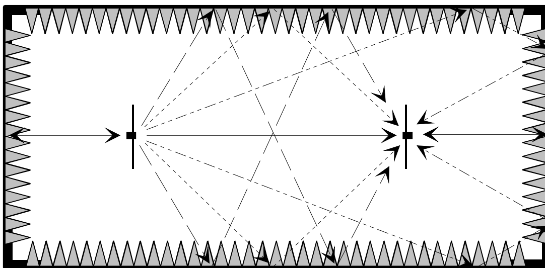
Figure 8: Plan view of an Anechoic Chamber with a Ground Plane which uses pyramidal absorber
