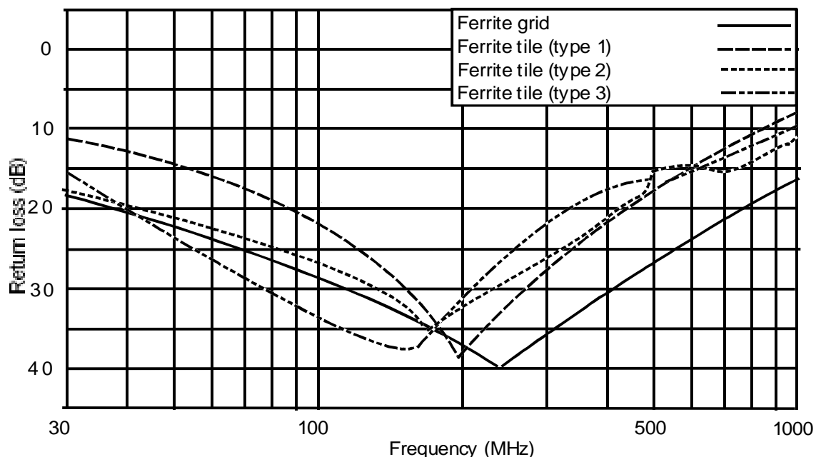
Figure 6: Normal incidence return loss variation of a ferrite grid and three different designs of ferrite tile against frequency
