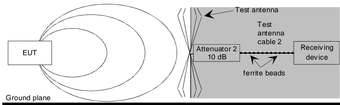
Figure 50: Stage 1: EUT measurement
