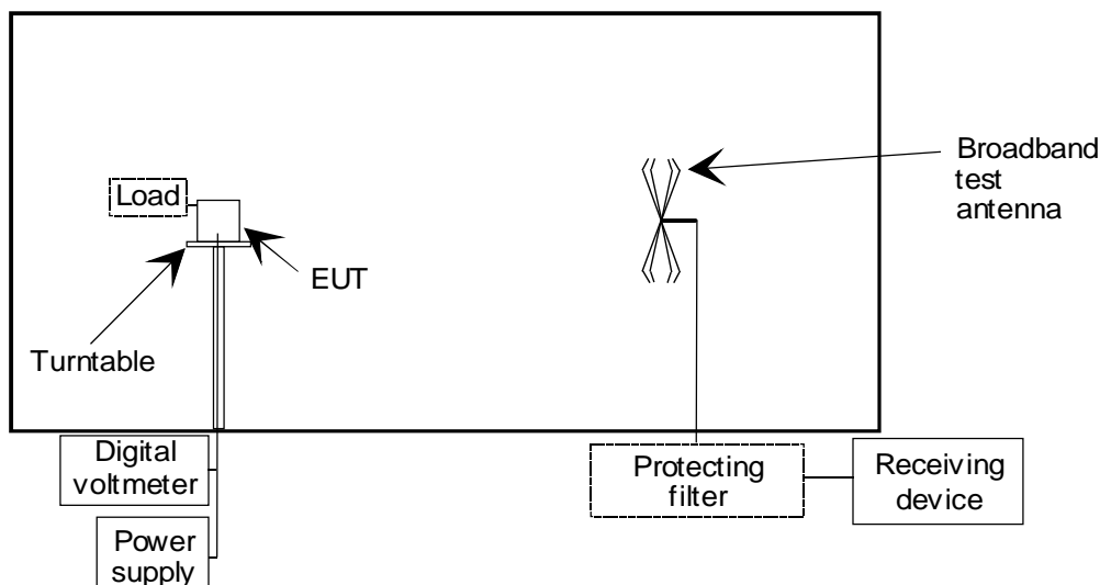
Figure 46: Elevation view of shielded chamber set up for the characterization tests
