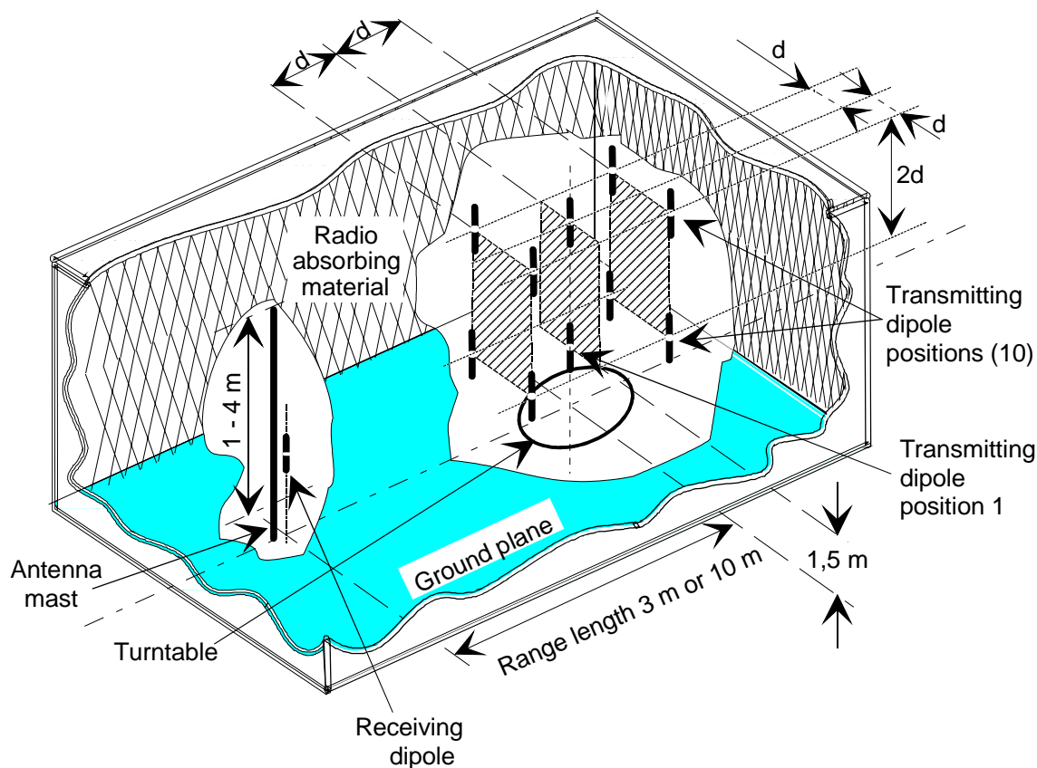
Figure 27: Antenna arrangements for vertical polarization
