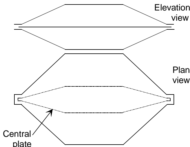
Figure 5: Open three-plate Stripline as detailed in IEC 604893 [3] Appendix J 1988
