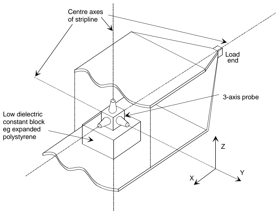
Figure 16: Location of the three-axis probe at the intersection of the Stripline's centre axes
