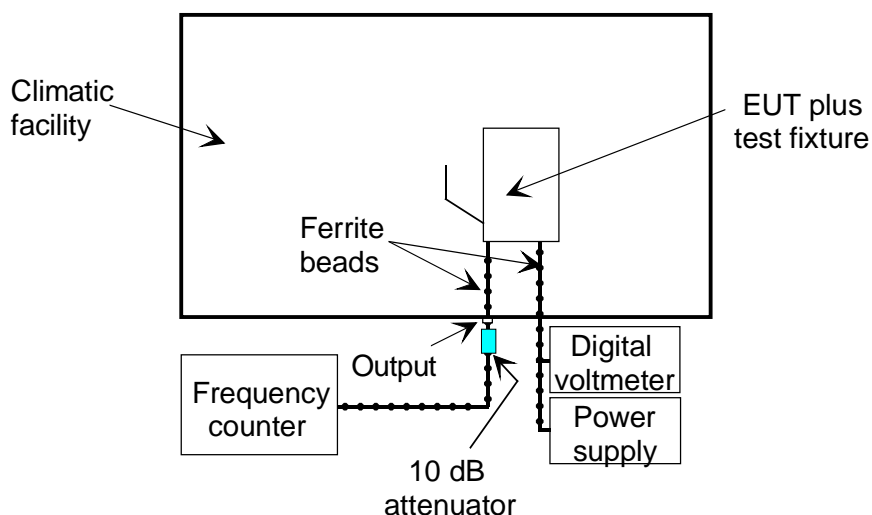
Figure 6: Set-up for frequency error measurement using a test fixture
