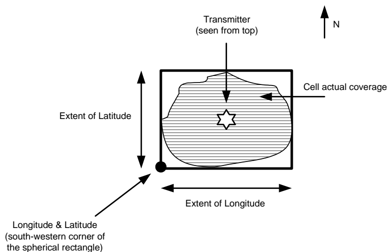
Figure 8.7: Cell coverage area in case of omnidirectional signal as defined in EN 300 468 [i.4]
