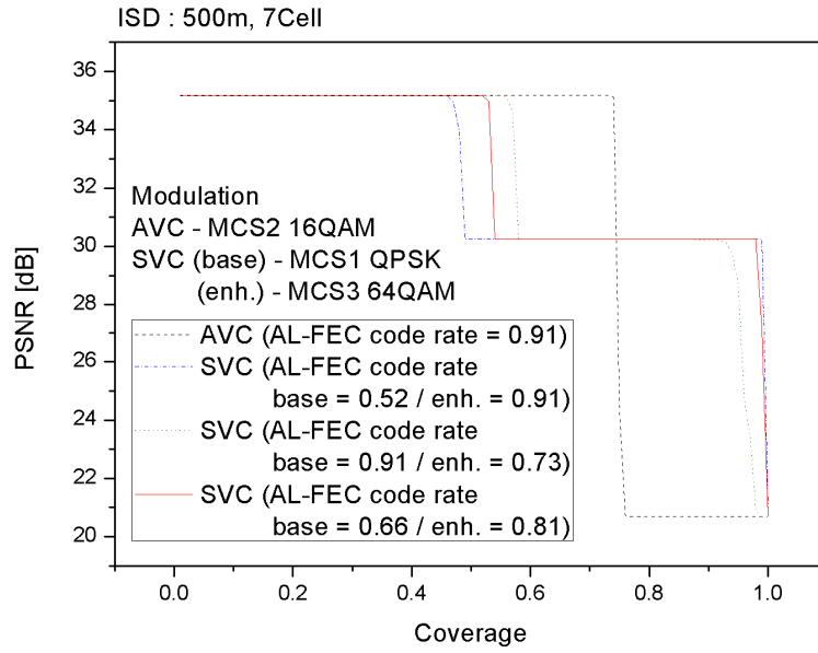
Figure 23: Comparison of PSNR curves of H.264/AVC and SVC
