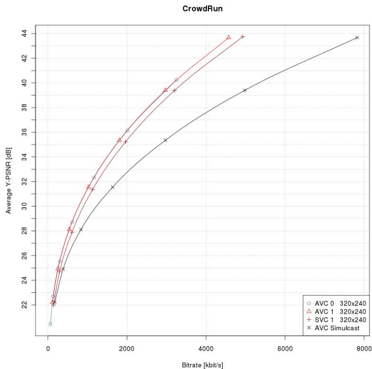
Figure 57: CrowdRun
