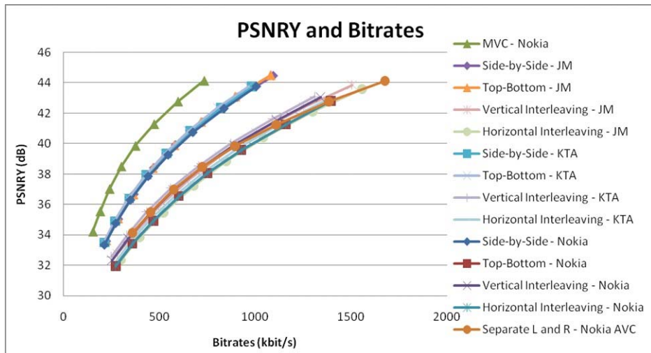
Figure 73: Book arrival
