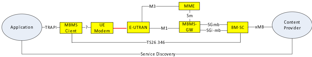
Figure 20: Architecture for Full MBMS Service Mode
