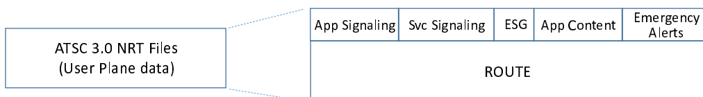
Figure 16: ATSC 3.0 NRT Service Protocol Stack over xMB-U
