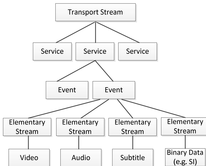
Figure 2: DVB Service Delivery Model
