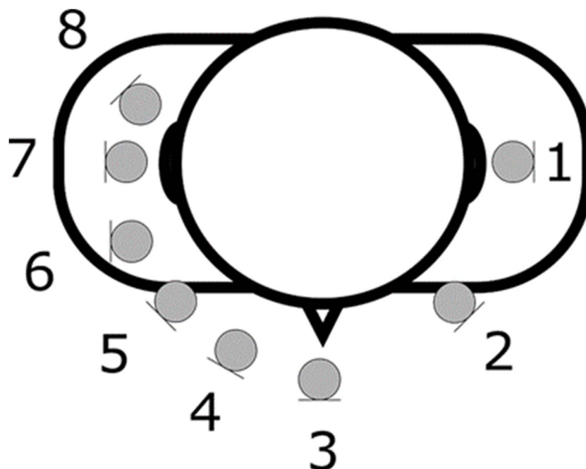
Figure 87: Microphone array for handset testing according to ETSI TS 103 224
