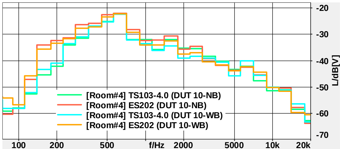
Figure 130: 1/3 rd octave band spectrum of noise-only time range of room#4 (Pub Noise)
