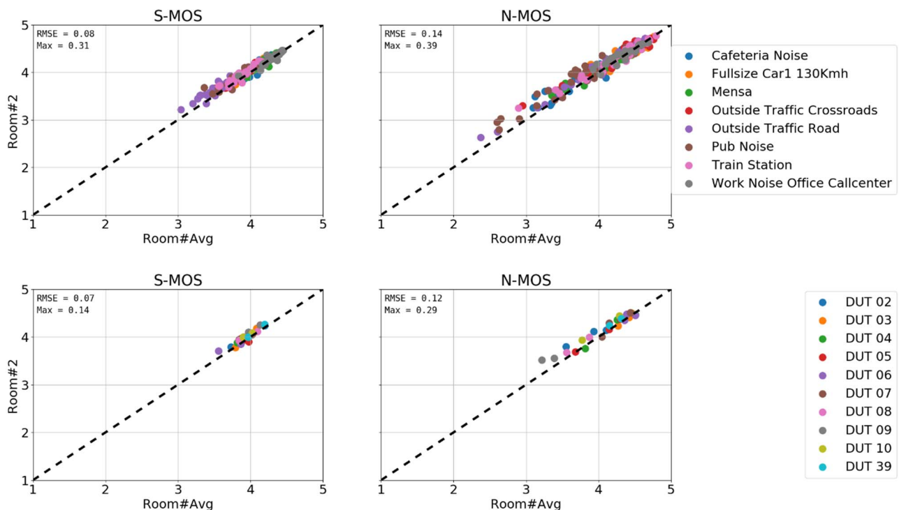
Figure 140: Comparison of Room#2 vs Room#Avg (TS103-4.1)
