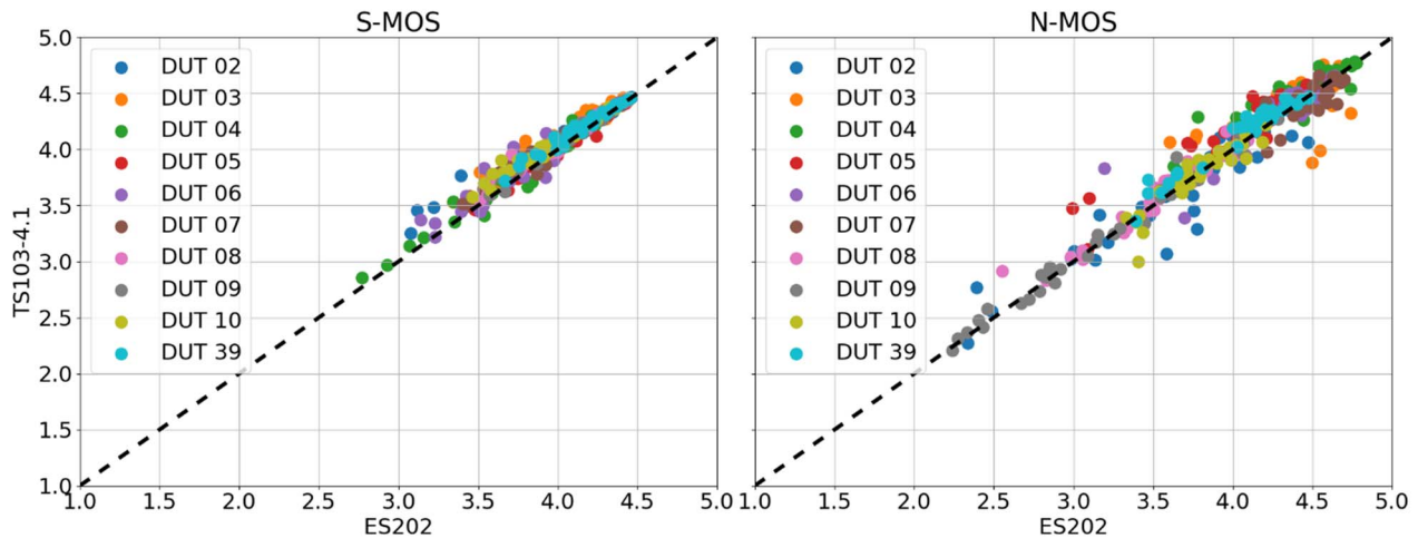
Figure 106: Results S-/N-MOS for TS103-4.1 vs. ES202 (NB)
