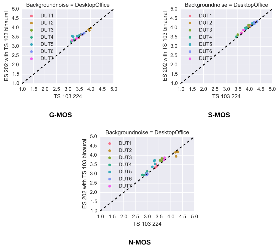
Figure 75: Correlation of G-MOS (WB) results between TS 103 224 and ES 202 396-1 methodology (noise from TS 103 224)
