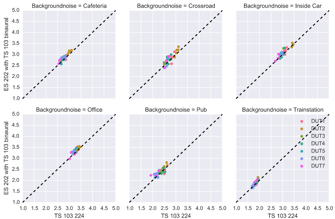
Figure 30: Correlation of G-MOS (WB) results between TS 103 224 and ES 202 396-1 methodology (noises from TS 103 224)
