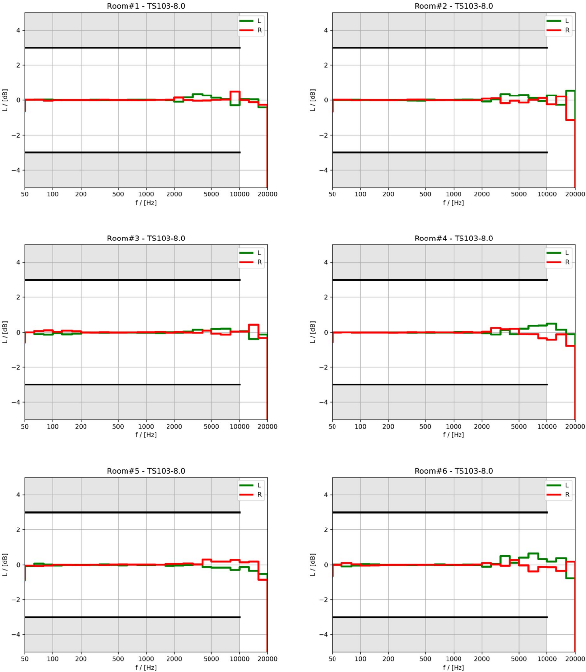
Figure 95: Validation results of equalization (TS103-8.0)
