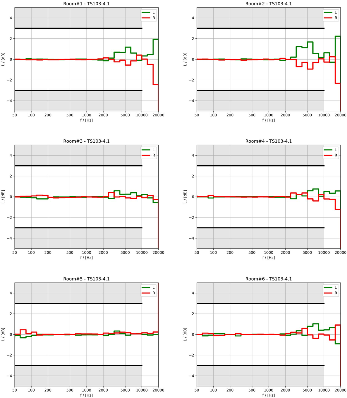
Figure 94: Validation results of equalization (TS103-4.1)
