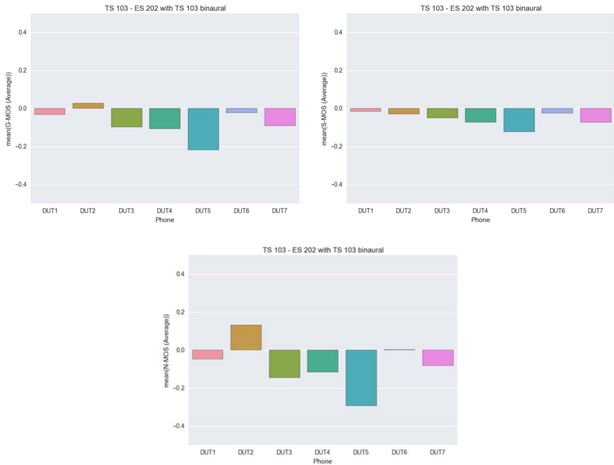
Figure 78: Differences (WB) between TS 103 224 and ES 202 396-1 methodology (binaural noises from TS 103 224 database)
