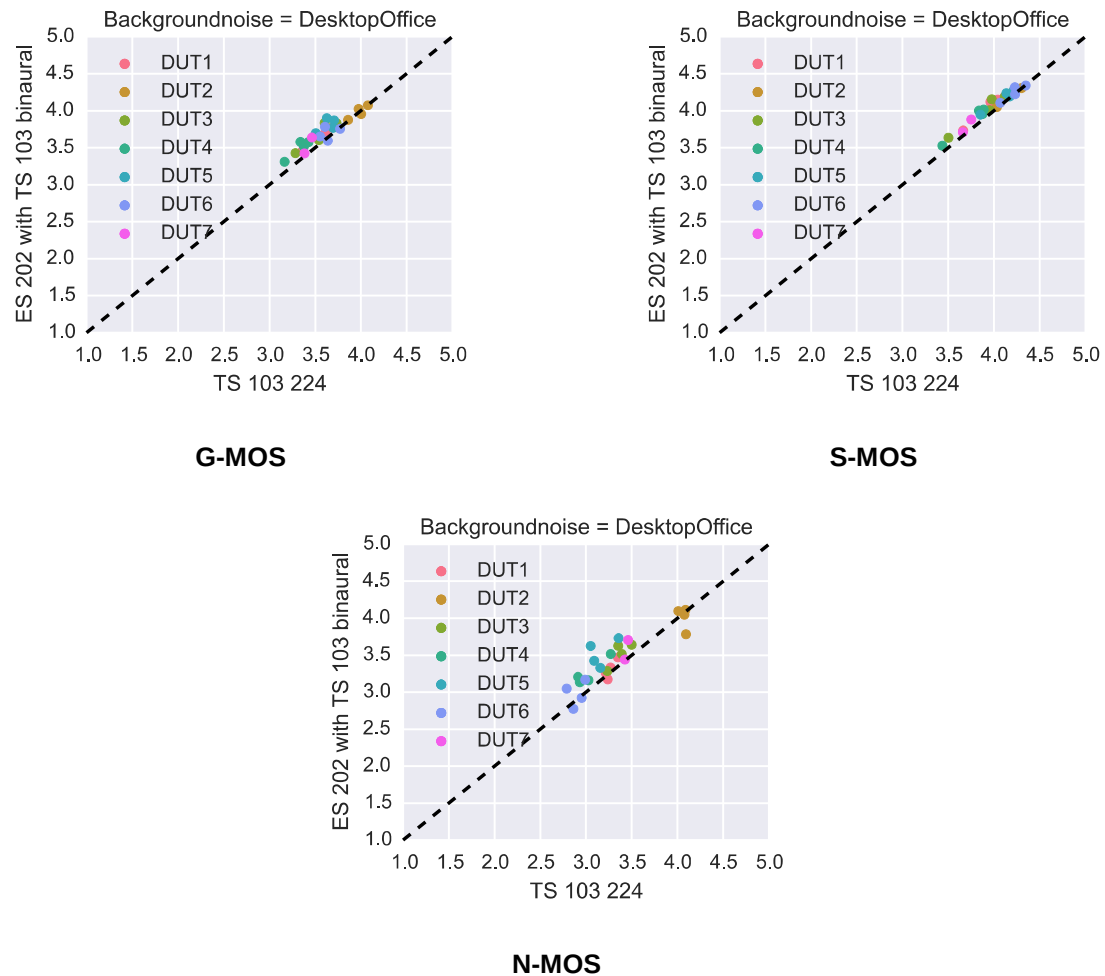
Figure 76: Correlation of G-MOS (NB) results between TS 103 224 and ES 202 396-1 methodology (noise from TS 103 224)
