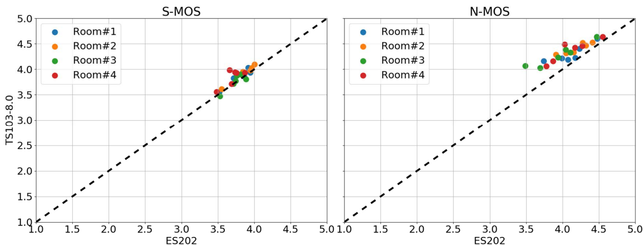
Figure 122: Average results S-/N-MOS for TS103-8.0 vs. ES202 (SWB)
