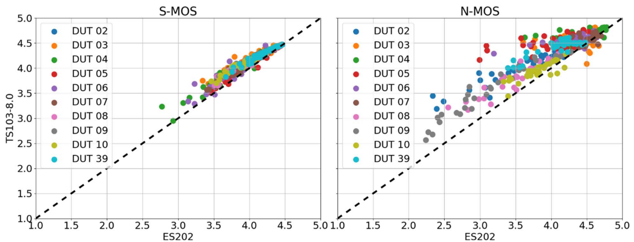
Figure 107: Results S-/N-MOS for TS103-8.0 vs. ES202 (NB)
