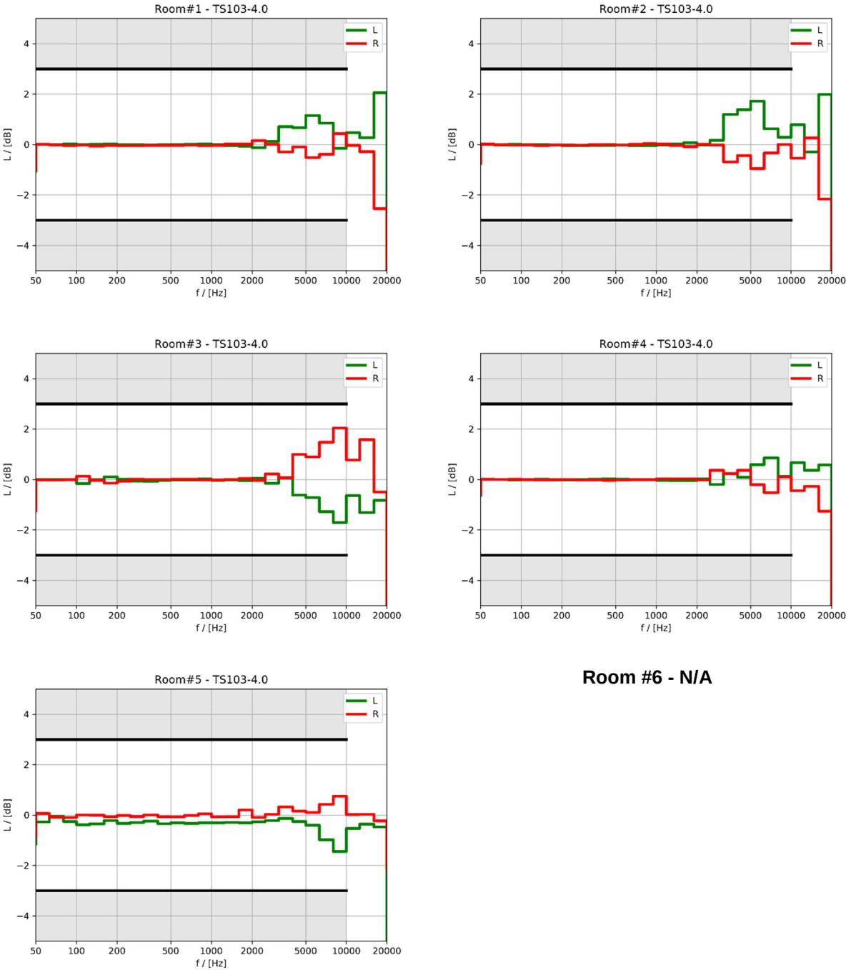
Figure 93: Validation results of equalization (TS103-4.0)
