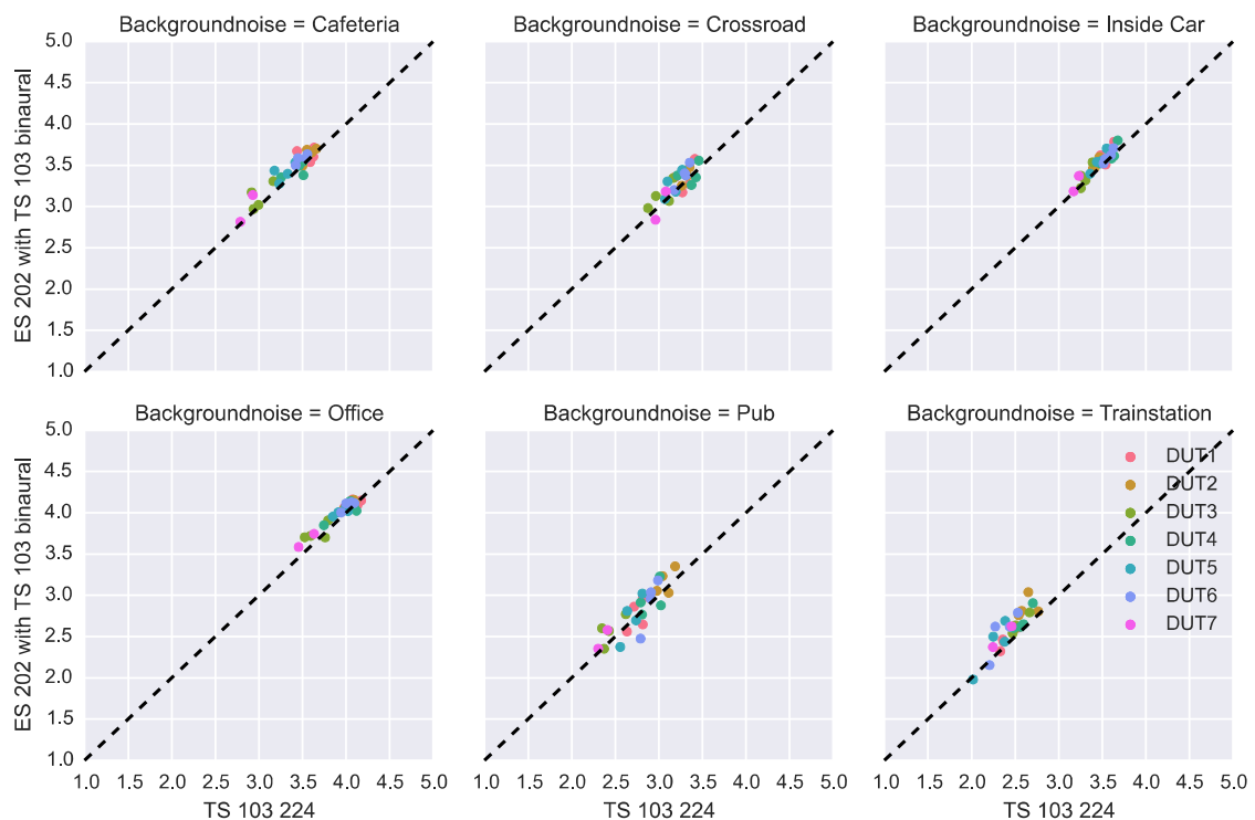
Figure 37: Correlation of S-MOS (NB) results between TS 103 224 and ES 202 396-1 methodology (noises from TS 103 224)
