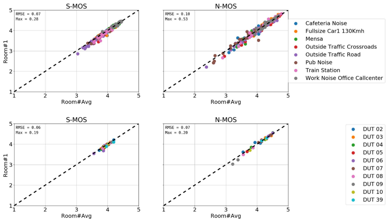
Figure 139: Comparison of Room#1 vs Room#Avg (TS103-4.1)
