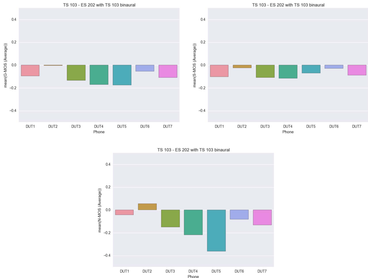
Figure 80: Differences (NB) between TS 103 224 and ES 202 396-1 methodology (binaural noises from TS 103 224 database)
