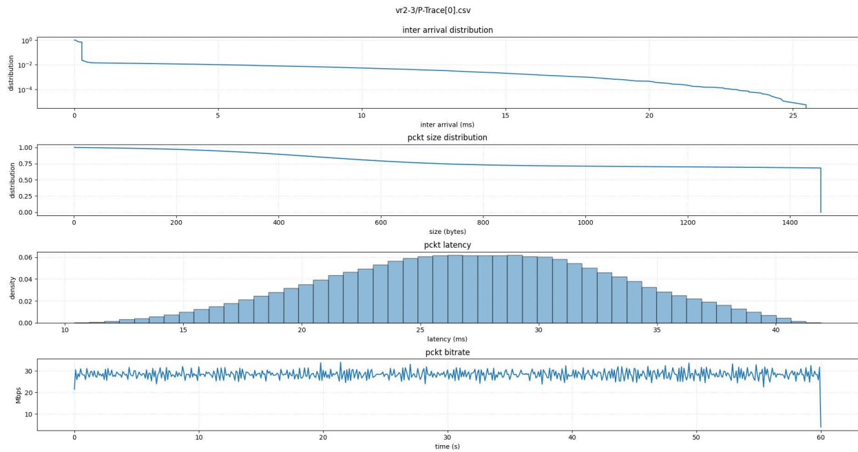
Figure 6.5.2-1 VR2-3 Statistics
