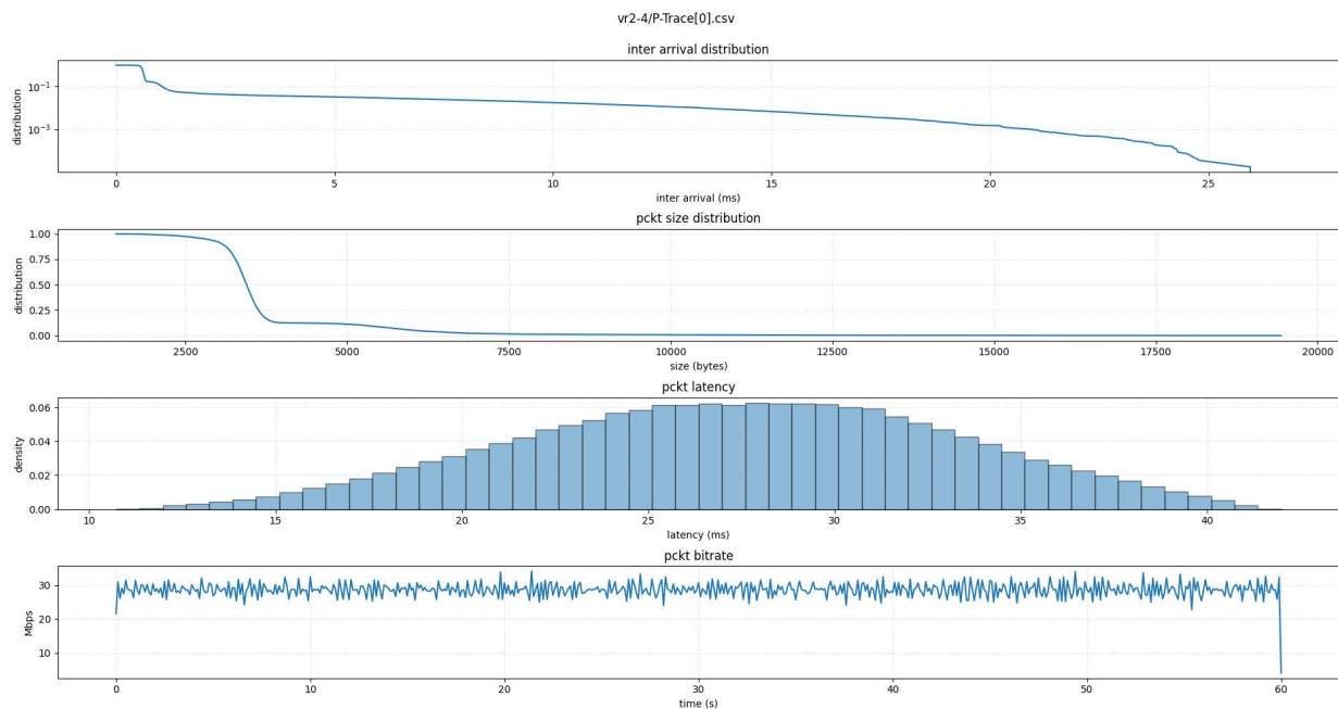
Figure 6.5.2-2 VR2-4 Statistics
