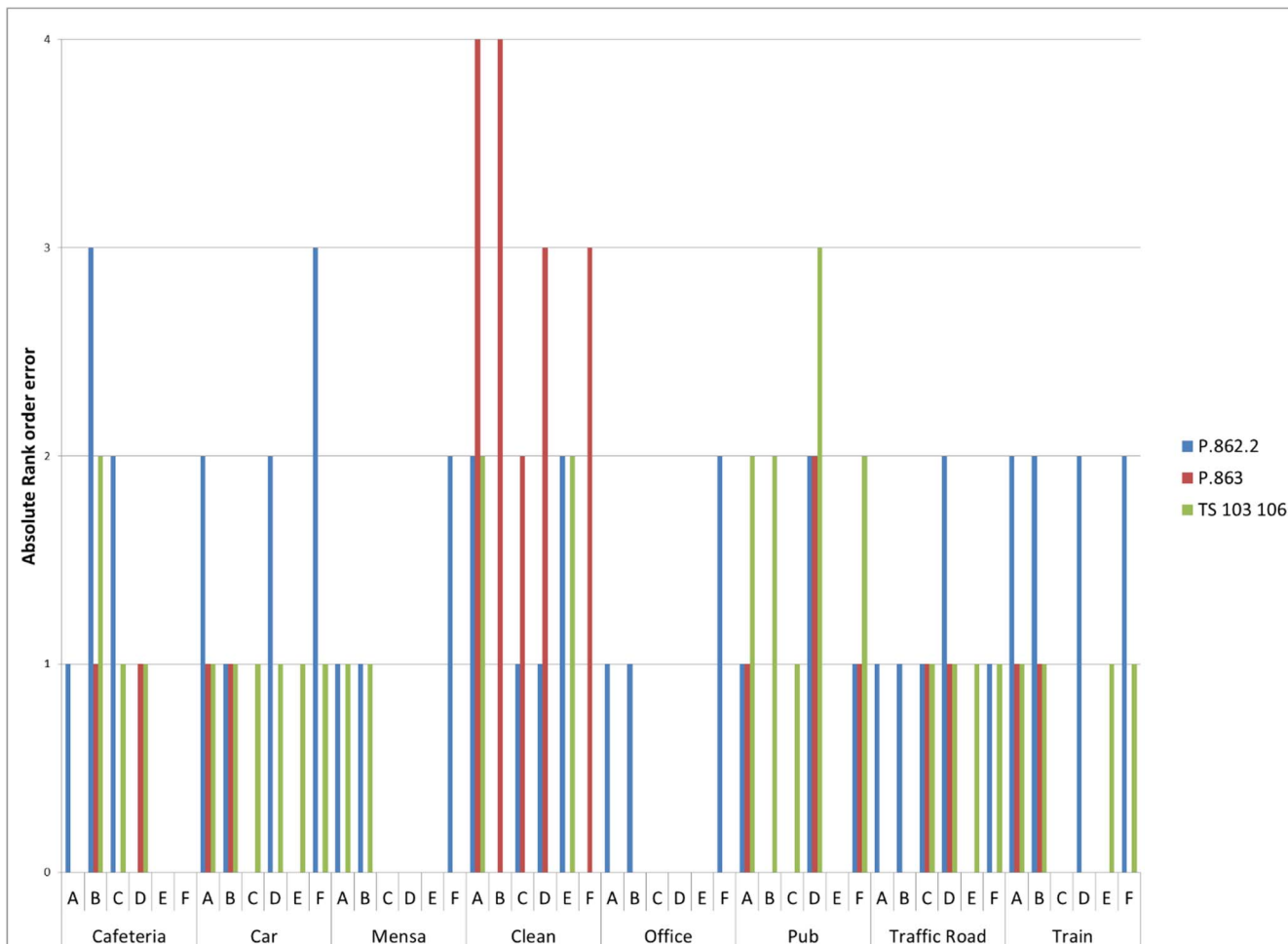
Figure 31: Rank Order Errors for each Objective Measure in WB
