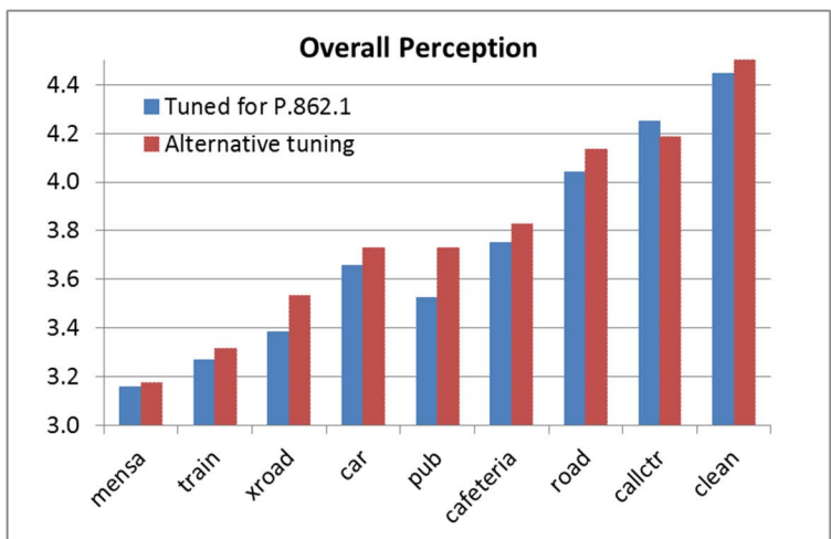
Figure 26: Results of Experiment 2 - P.835 [4] Overall Score
