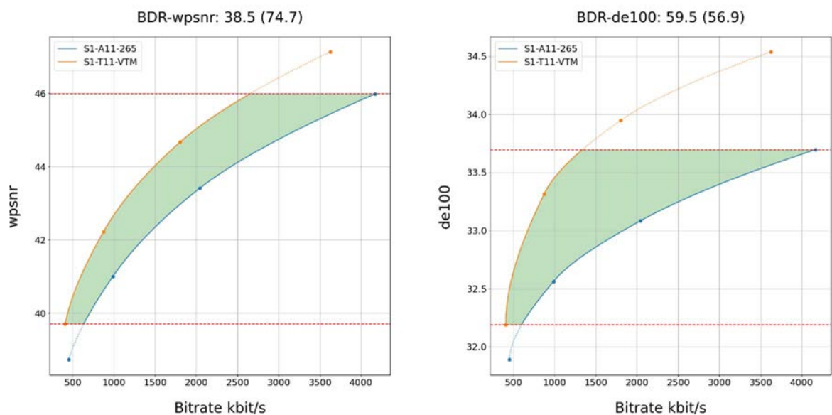
Figure 8.2.4.2-2 Rate-Quality curves and BD rate gain for wpsnr and de100 of H.266/VVC VTM with S1-VTM-02 against H.265/HEVC HM with configuration S1-HM-02 for reference sequence S1-R11
