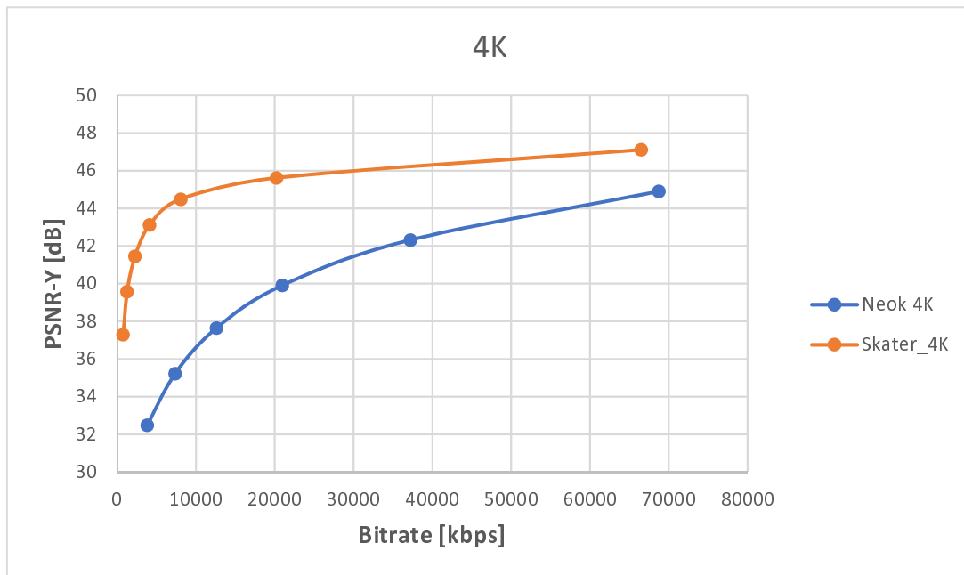
Figure C. 5.1.3-2: R-D curves for 4K sequences.
