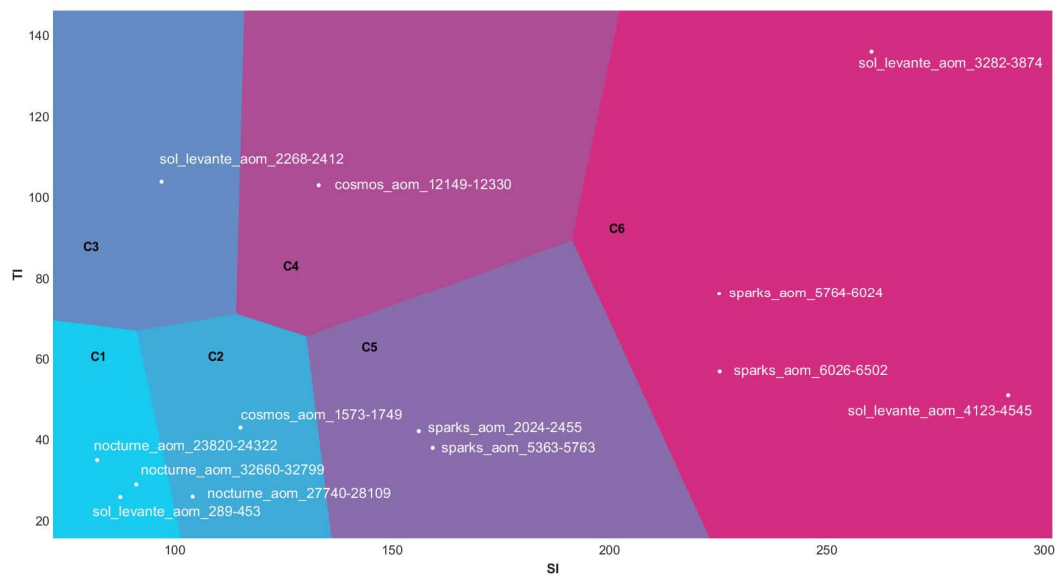
Figure C.3.2.2.5-1: SI-TI clustering for the challenging HDR sequences (6 clusters)
