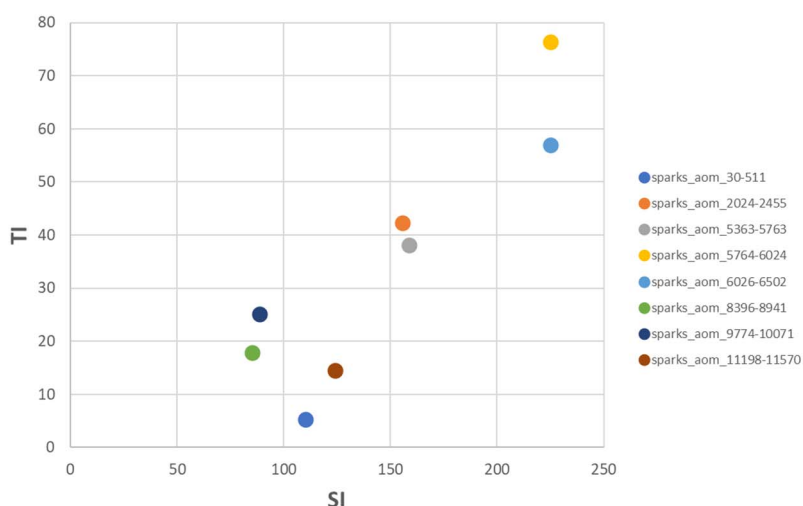
Figure C.3.2.2.3-1: SI-TI for the AOM dataset (Sparks clips)
