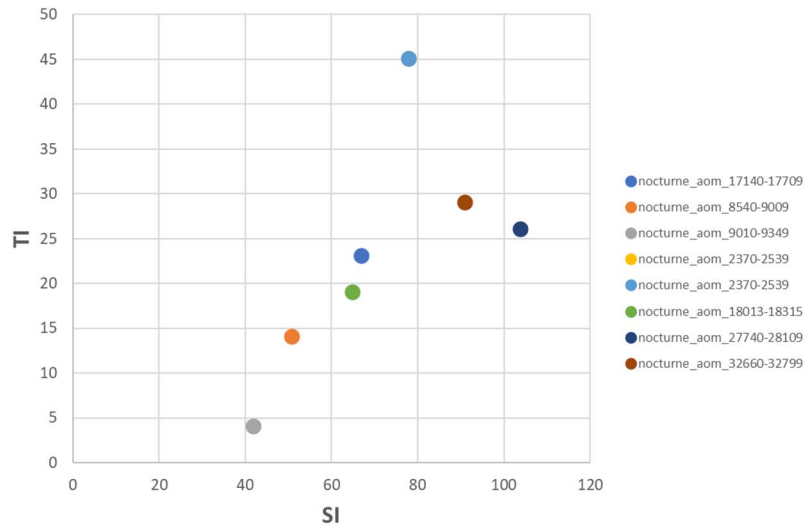
Figure C.3.2.2.3-3: SI-TI for the AOM dataset (Nocturne clips)
