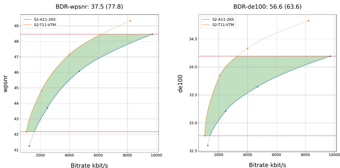
Figure 8.2.4.3-2 Rate-Quality curves and BD rate gain for wpsnr and de100 of H.266/VVC VTM with S2-VTM-02 against H.265/HEVC HM with configuration S2-HM-02 for reference sequence S2-R11
