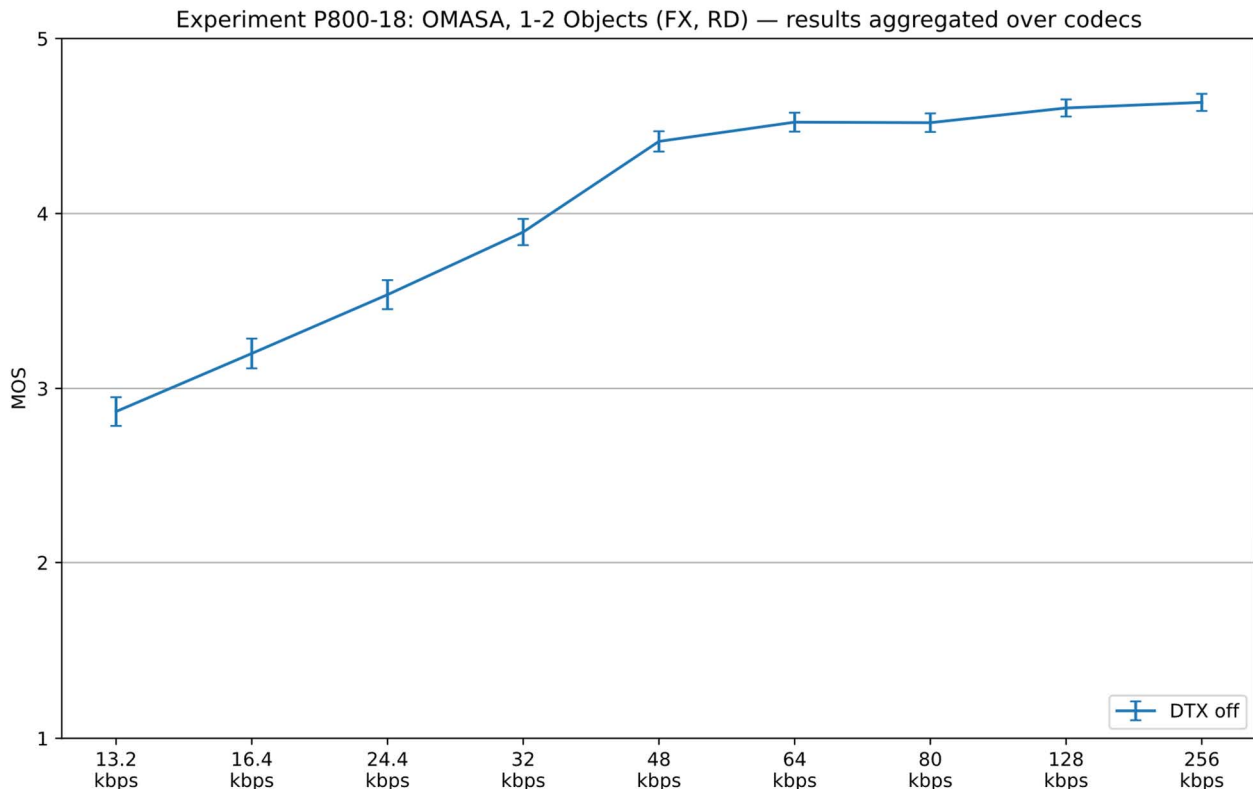
Figure 9.8-3: results aggregated over FX/FL for experiment P800-18
