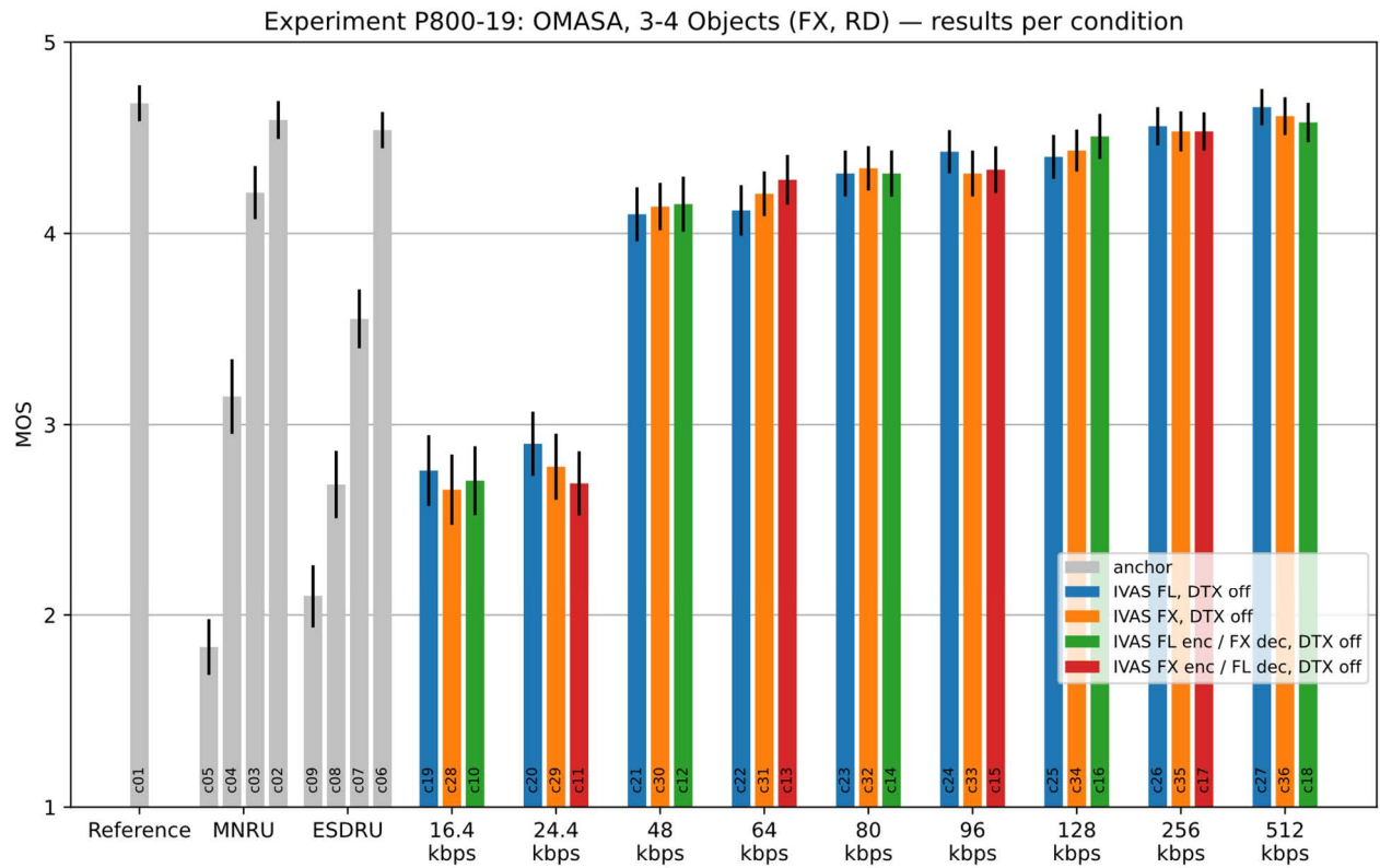
Figure 9.8-4: results per condition for experiment P800-19
