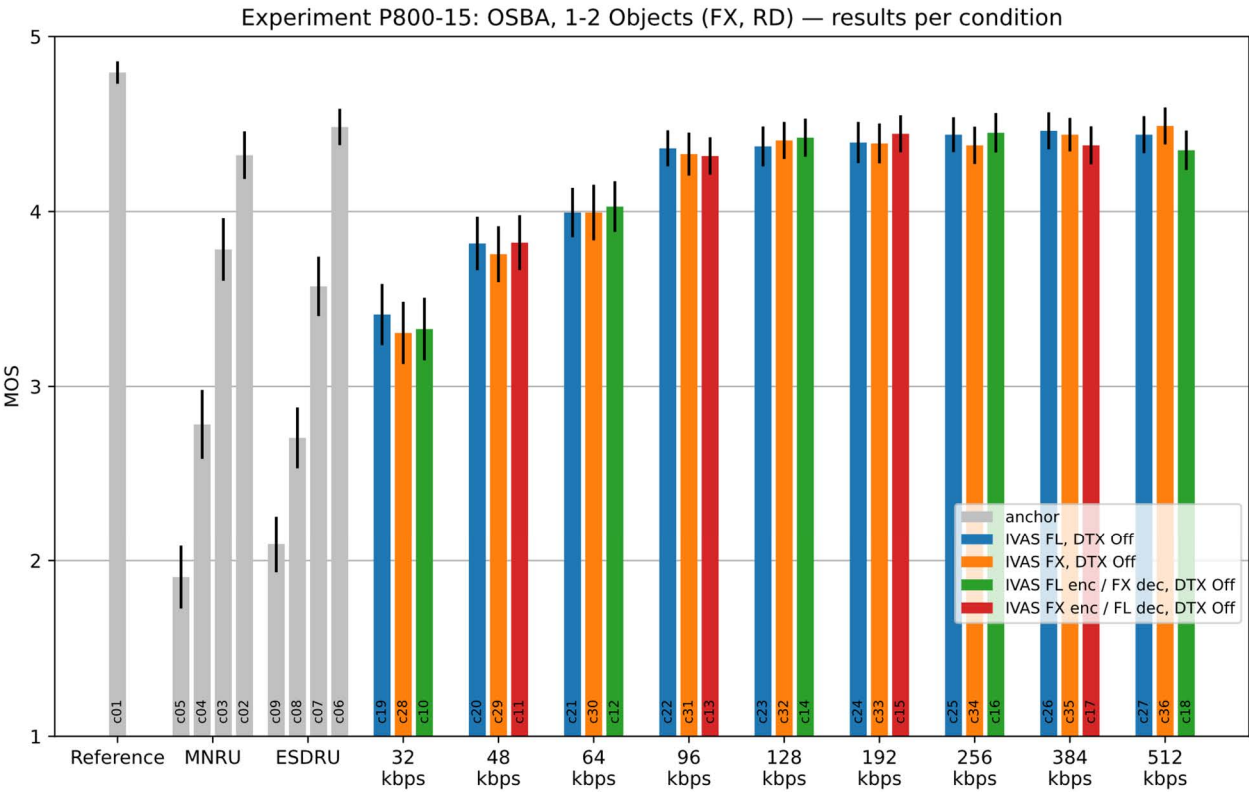
Figure 9.7-3: results per condition for experiment P800-15
