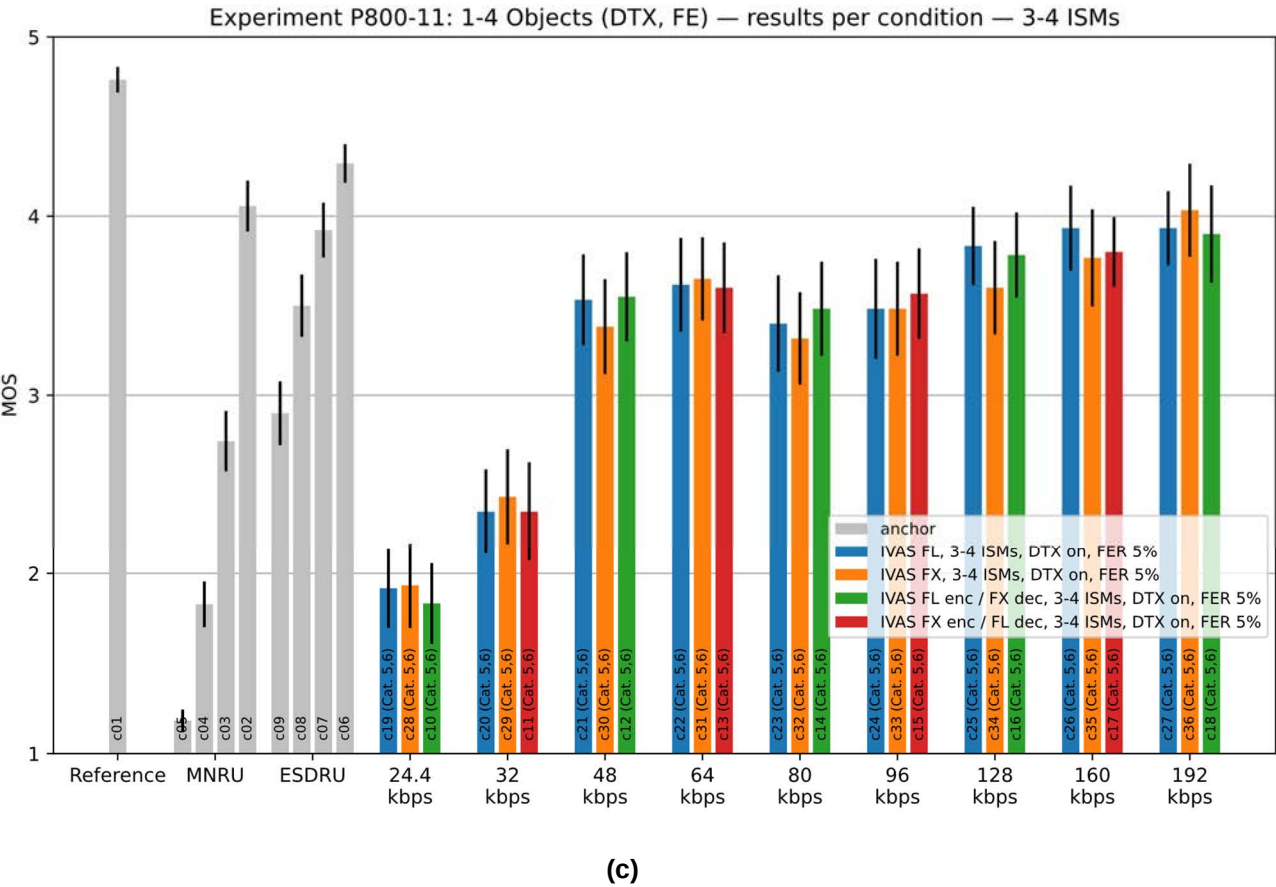
Figure 9.4-9: results per condition for experiment P800-11
