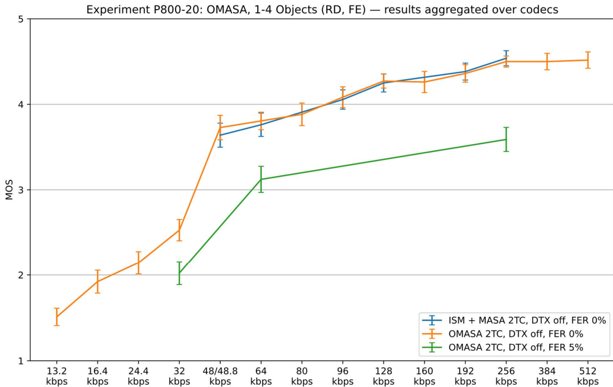
Figure 9.8-7: results aggregated over FX/FL for experiment P800-20
