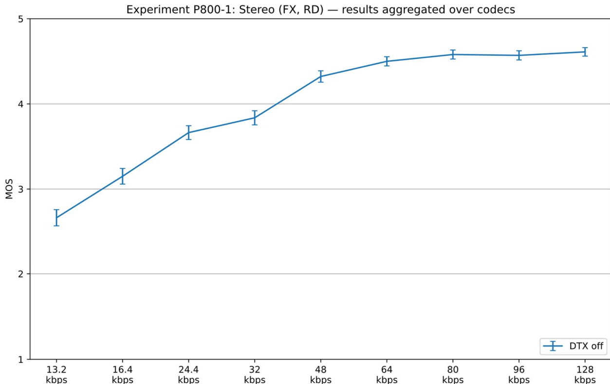
Figure 9.2-7: results aggregated over FX/FL for experiment P800-1
