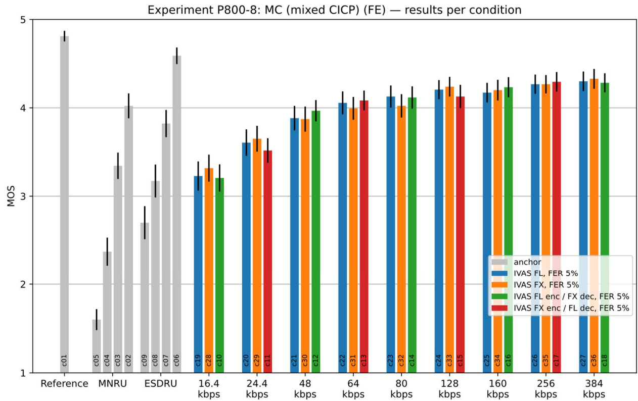
Figure 9.6-10: results per condition for experiment P800-8
