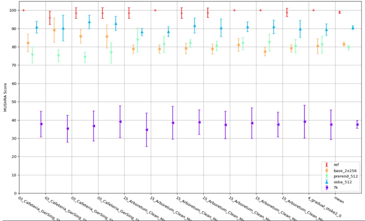
Figure 9.7-2: BS.1534 comparison between combined vs. separate operation of ISM + SBA at 512 kbps
