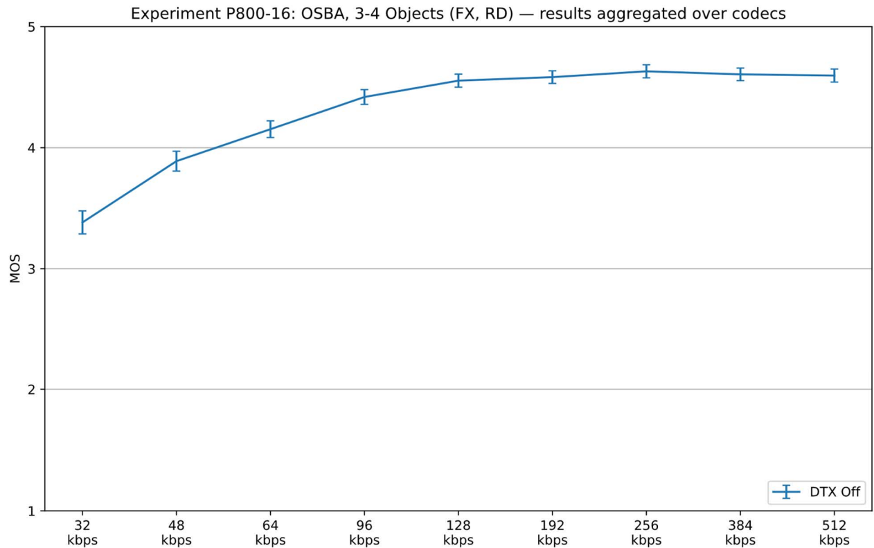
Figure 9.7-6: results aggregated over FX/FL for experiment P800-16
