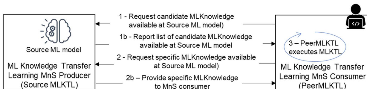
Figure 5.1.12.2.2-1: Scenario 1 - Interactions for ML-Knowledge Transfer Learning (MLKLT) to support training at the ML knowledge Transfer MnS consumer - the ML knowledge Transfer MnS consumer obtains the ML knowledge which it then uses for training the new ML model based on knowledge received from the MLKLT source MnS producer
