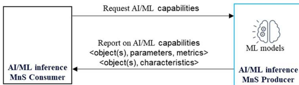
Figure 5.1.8.4-1: AI/ML capability request and report
