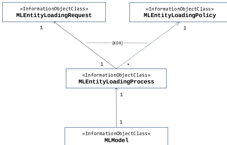
Figure 5.2.4.4.1-1: Example of ML model loading related NRMs
