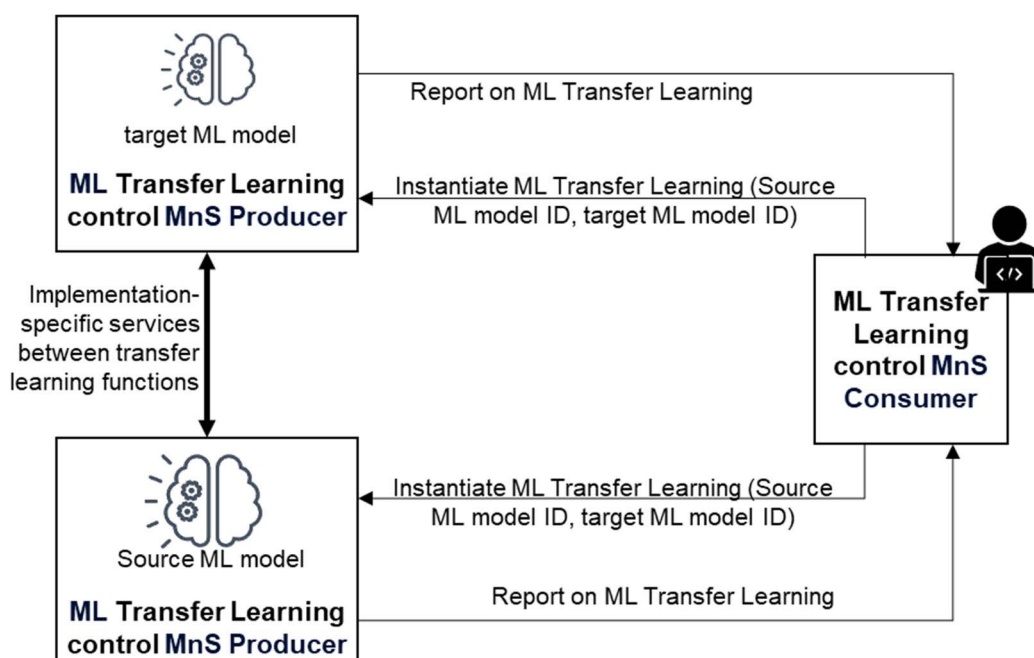
Figure 5.1.12.1-1: ML Knowledge Transfer Learning (MLKLT) flow between the source MLKLT (which is the entity with the pre-trained ML model), the peer MLKLT (which is the entity that shall train a new ML model) and the MLKLT MnS consumer (which may be the operator or another management function that wishes to trigger or control MLKLT)
