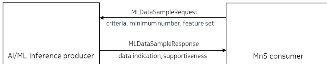
Figure 5.1.4.4.2-1: Interaction between AI/ML inference MnS producer and MnS consumer (e.g. the ML training function) to support efficient re-training of ML model
