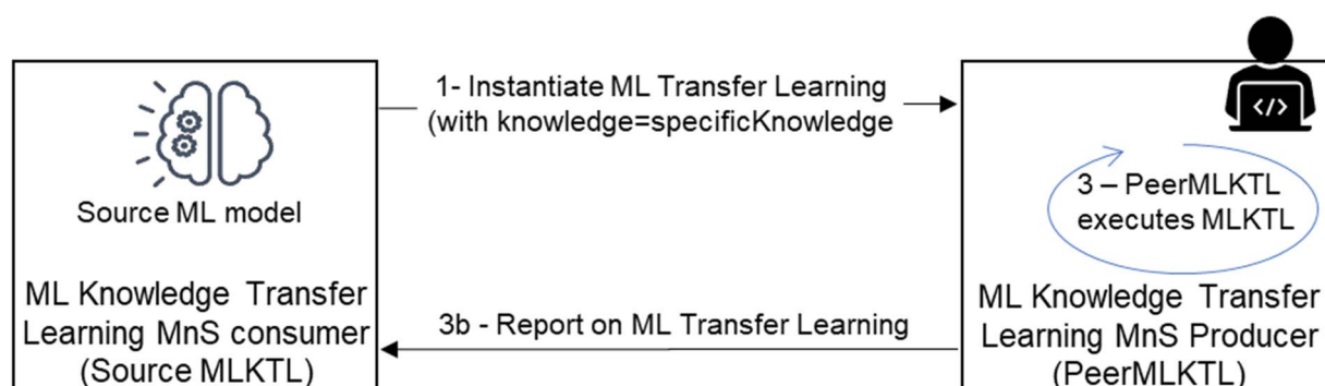
Figure 5.1.12.2.2-2: Scenario 2 - interactions for ML-Knowledge Transfer Learning (MLKTL) to support training at the ML knowledge transfer MnS consumer triggered by the MLKTL Source - the ML Transfer Learning MnS consumer acting as the MLKTL Source (the source of the ML knowledge) triggers the training at the ML knowledge Transfer MnS consumer by providing the ML knowledge to be used for the training, the ML Transfer Learning MnS consumer then undertakes the training
