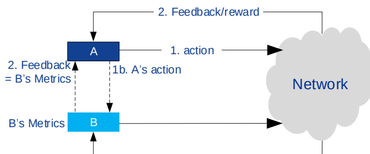
Figure 5.2.2.2-1: Distributed coordination of Cognitive Network Automation Functions (NAF)
