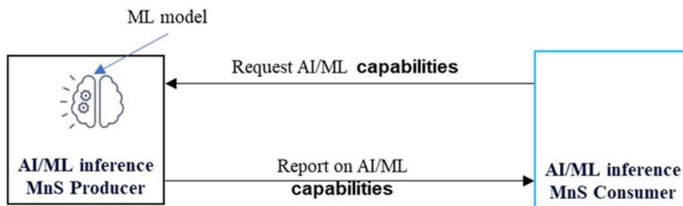
Figure 5.1.8.2.1-1: Request and reporting on AI/ML capabilities
