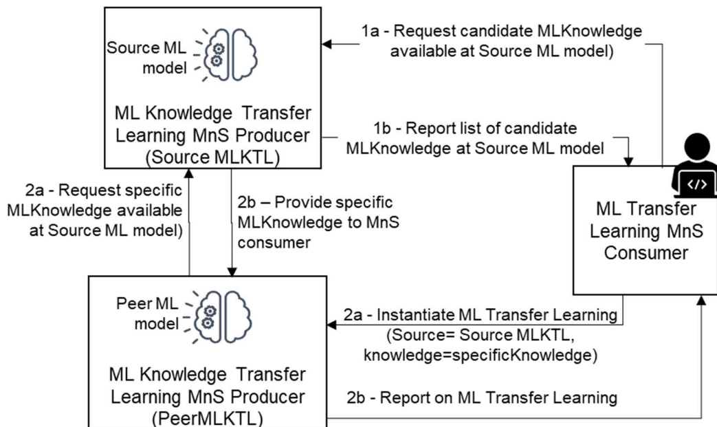
Figure 5.1.12.2.2-3: Scenario 3 - interactions for ML-Knowledge Transfer Learning (MLKLT) to support training at the Peer ML knowledge Transfer MnS producer who is different from the ML knowledge Transfer MnS consumer - the ML knowledge Transfer MnS consumer triggers training at the MLKLT peer MnS producer. The MLKLT MnS consumer then obtains the ML knowledge from the MLKLT source MnS producer and then uses the knowledge for training the new ML model based on knowledge received from the MLKLT source MnS producer
