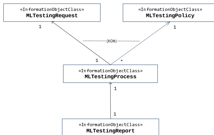
Figure 5.1.3.4.1-1: Example of ML model testing related NRMs
