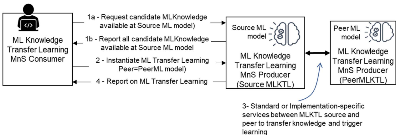
Figure 5.1.12.2.2-4: Scenario 4 - interactions for ML-Knowledge Transfer Learning (MLKLT) to support training at the Source ML knowledge Transfer MnS producer - the ML knowledge Transfer MnS consumer triggers training at the MLKLT source MnS producer. The MLKLT MnS consumer then obtains the ML knowledge from the MLKLT source MnS producer and then uses the knowledge for training the new ML model based on knowledge received from the MLKLT source MnS producer
