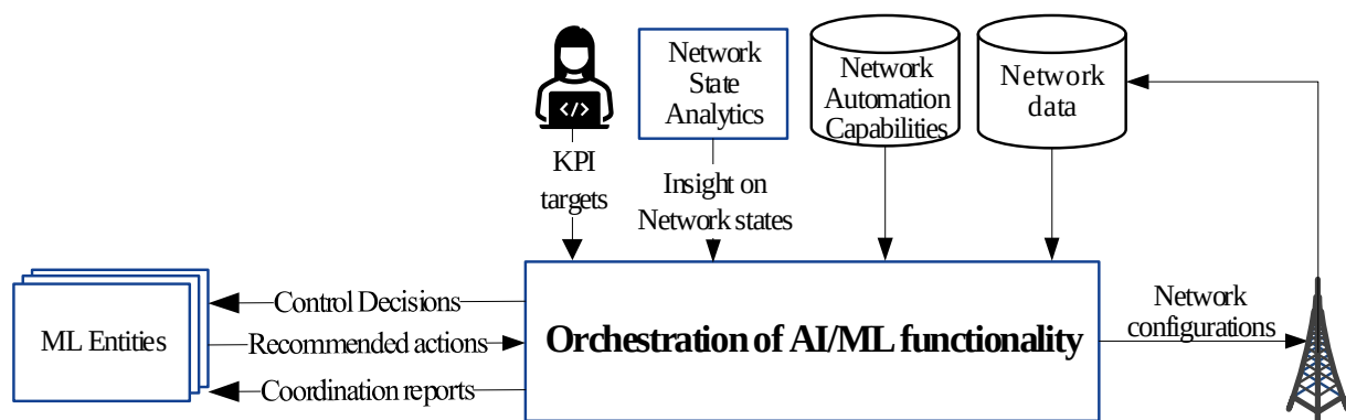
Figure 5.2.2.2.5-1: Orchestrating AI/ML
