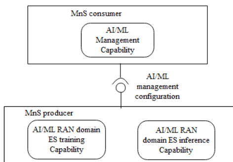
Figure 5.2.7.2.1-1: ML model configuration initiated by MnS consumer
