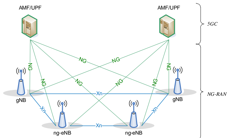
Figure 4.4.1.2-1: NG-RAN Overall Architecture
