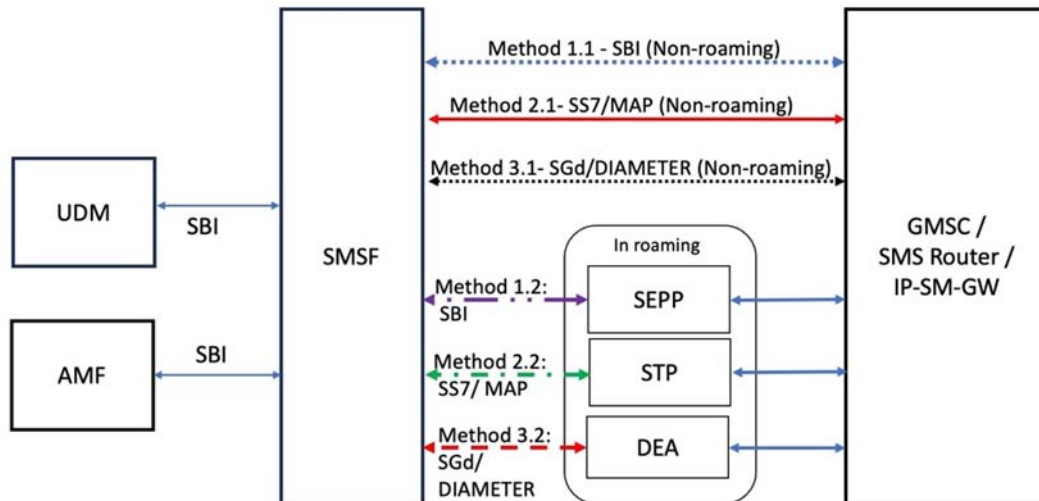
Figure Y.2.1-1: Interface connections between SMSF and other network entities
