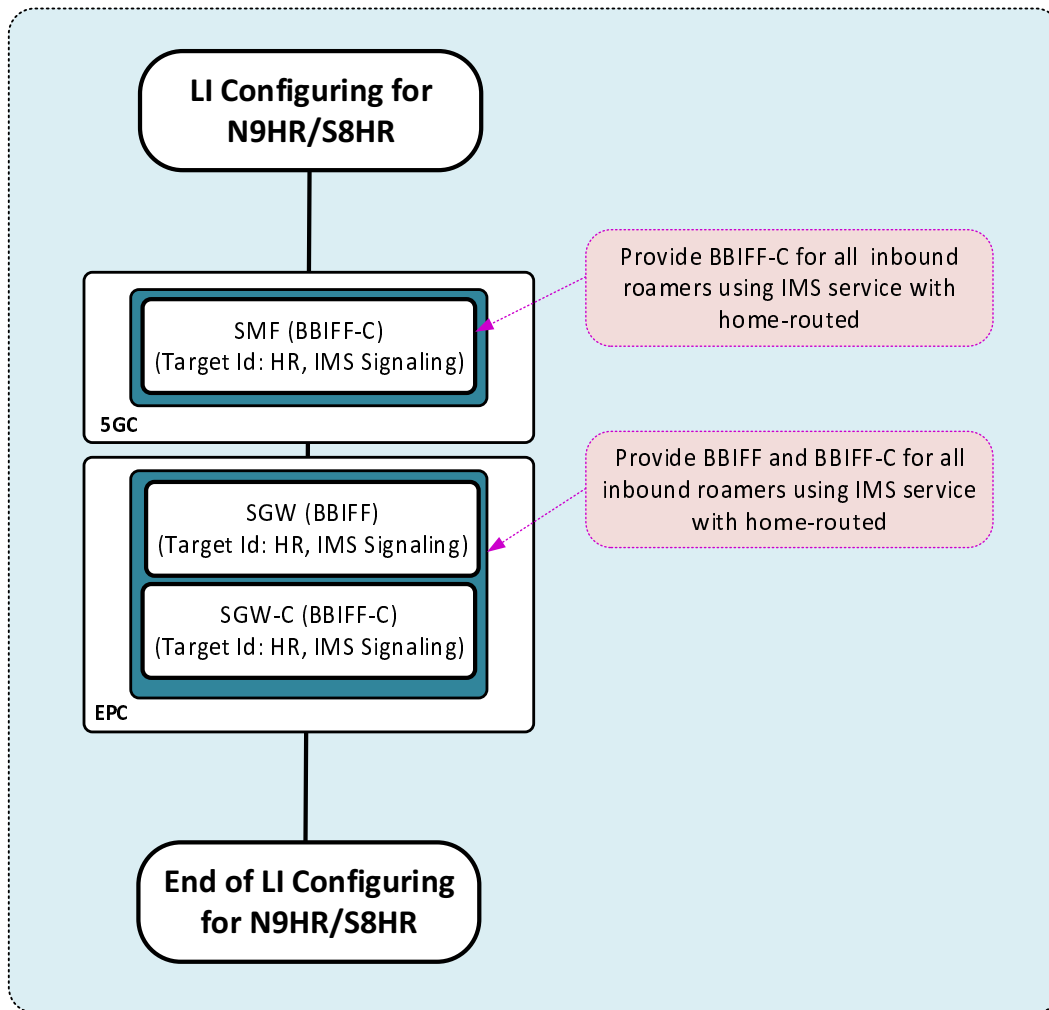
Figure 5.5.2-1: LIPF logic for initial configuration for N9HR/S8HR
