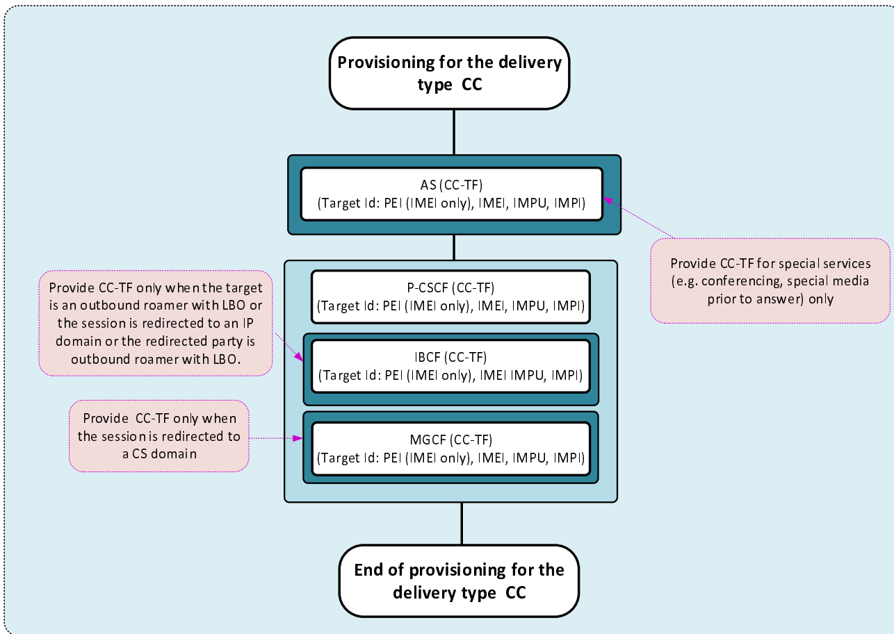
Figure 5.5.4.1-3: LIPF logic for delivery type of CC for service type of Voice when target is not a non-local ID
