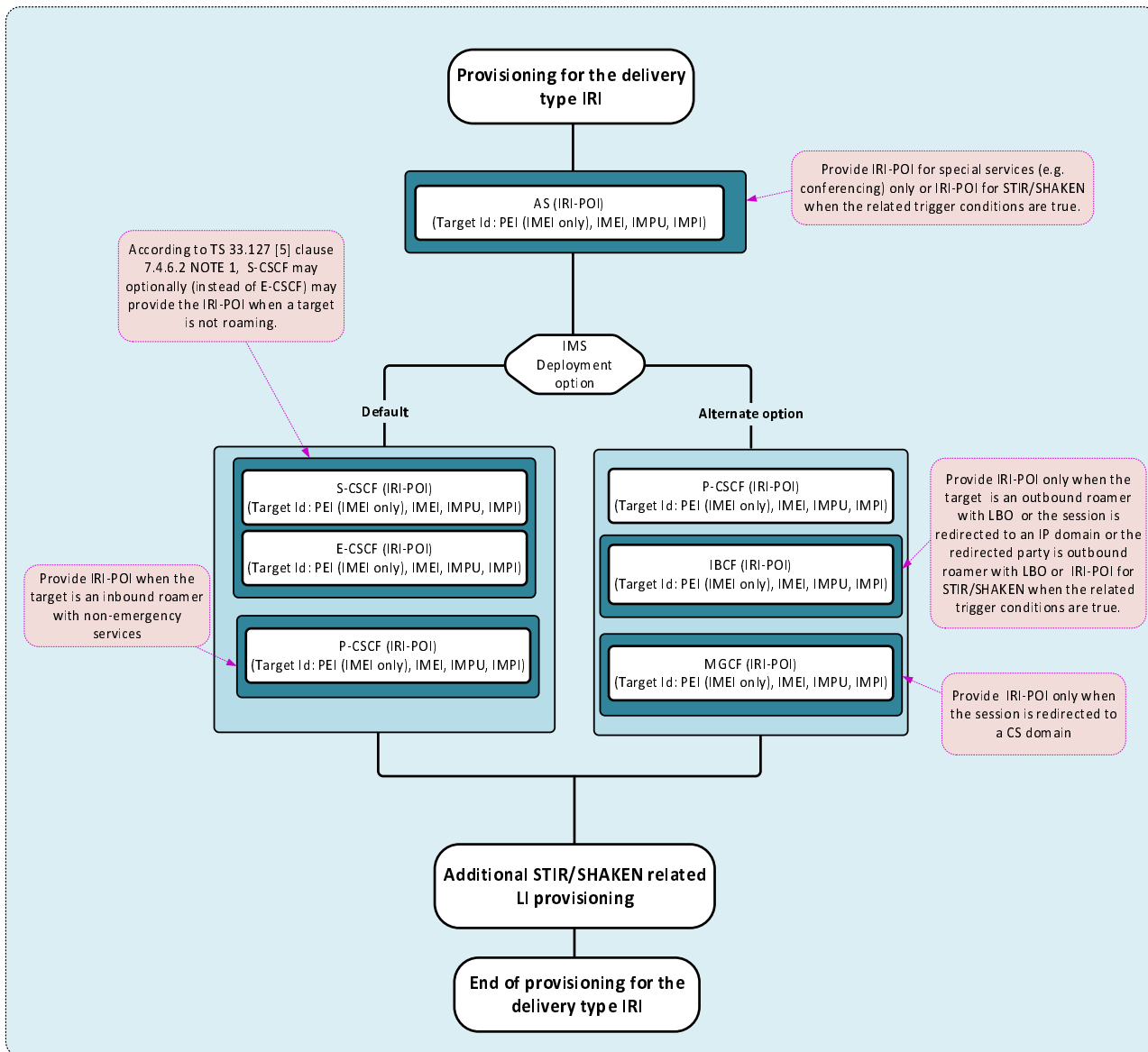
Figure 5.5.4.1-2: LIPF logic for delivery type of IRI for service type of Voice when target is not a non-local ID
