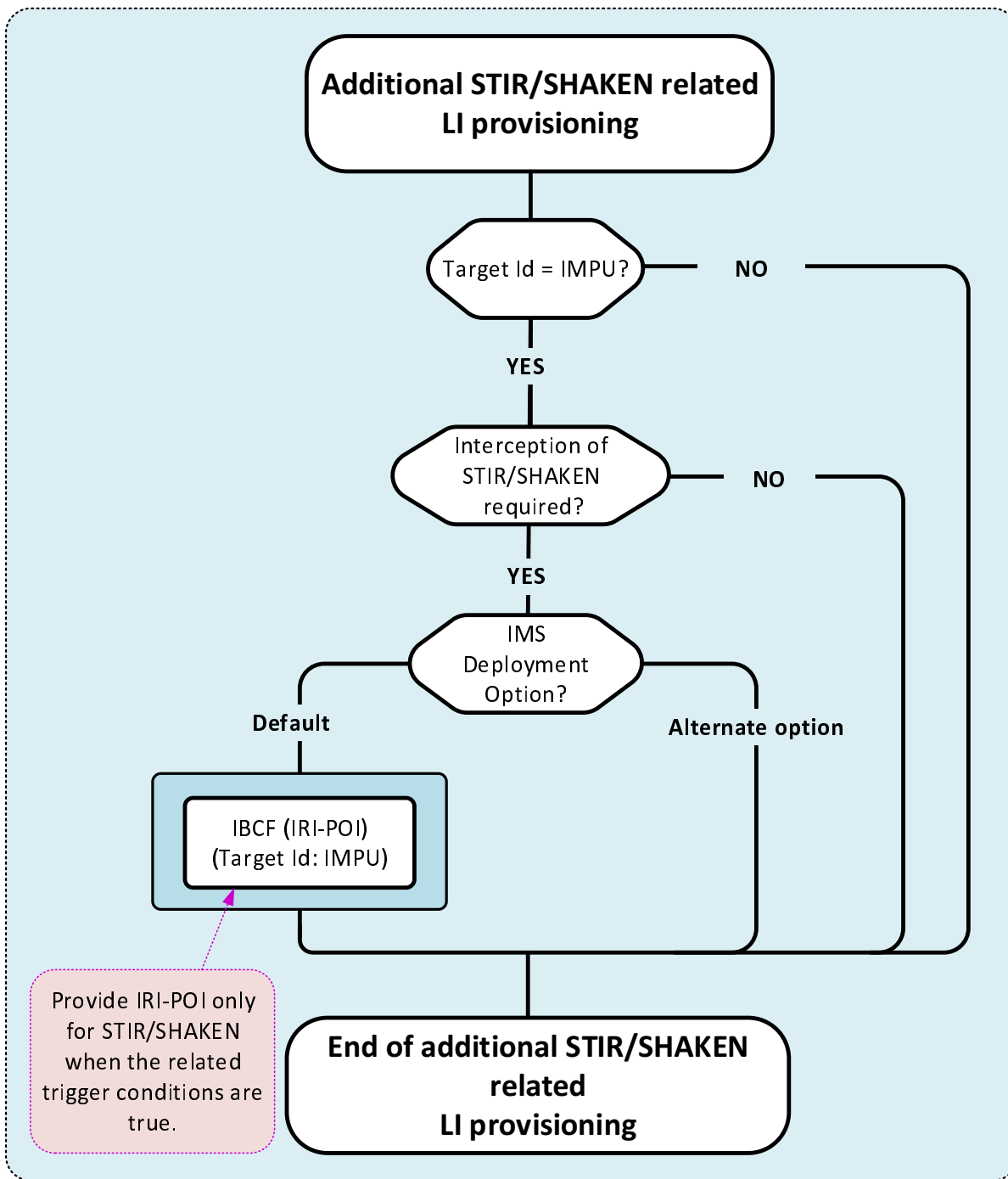
5.5.4.1-5: LIPF logic for additional STIR/SHAKEN related provisioning
