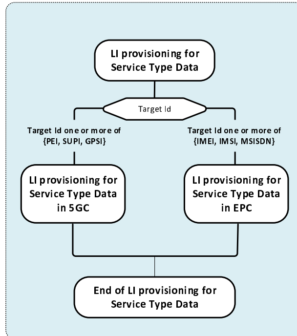
Figure 5.4.2-1: Top-level view of LIPF logic for the service type Data
