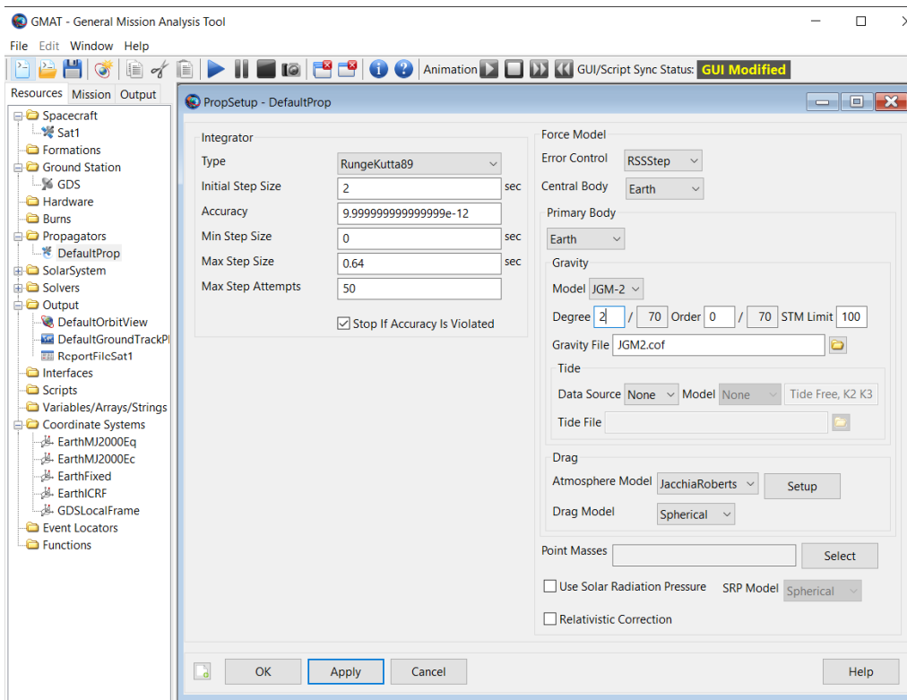
Figure 5.2.4-2: Propagator Setting for NGSO Satellites
