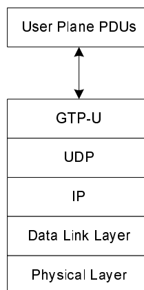
Figure 5.4.3.1-1: NG-U Protocol Stack
