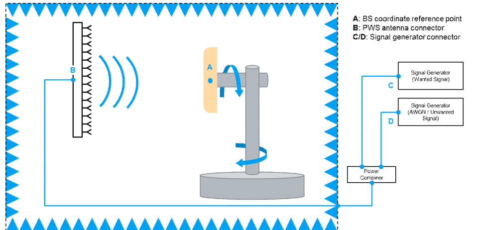
Figure 7.6.1-3: PWS measurement setup, OTA dynamic range, ACS, blocking and ICS
