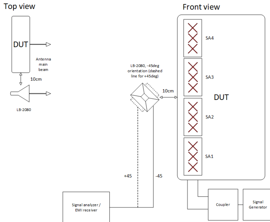
Figure 6.4.4.4-1: Co-located horn antenna example measurement setup
