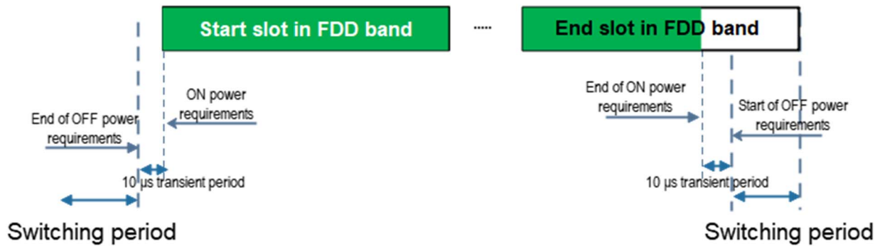
Figure 5.3.2-1: ON/OFF time mask for NR UL transmission for DL CA via switching with non-CA in the UL
