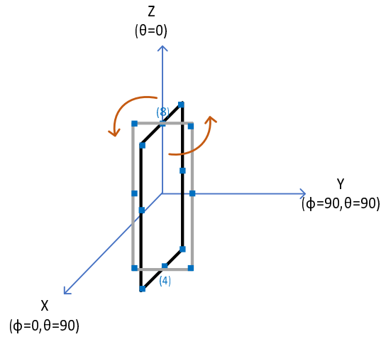
Figure 7.3-4: Example of UT rotation of \Omega_{UT,\alpha} = 0 - 360 degrees, \Omega_{UT,\beta} = 90 degrees, \Omega_{UT,\gamma} = 0 degrees
