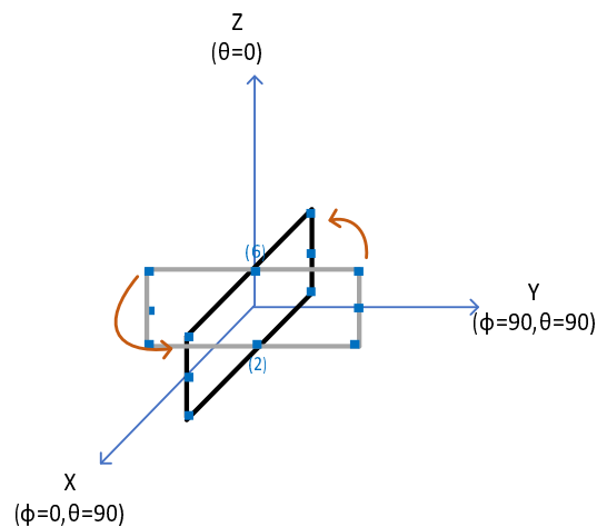
Figure 7.3-5: Example of UT rotation of \Omega_{UT,\alpha} = 0 - 360 degrees, \Omega_{UT,\beta} = 0 degrees, \Omega_{UT,\gamma} = 90 degrees
