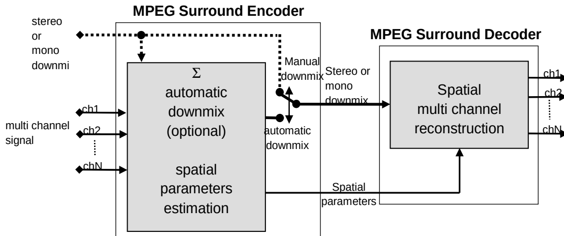
Figure 3: Principle of MPEG Surround, the downmix is coded using MPEG-4 AAC, HE AAC or HE AAC v2
