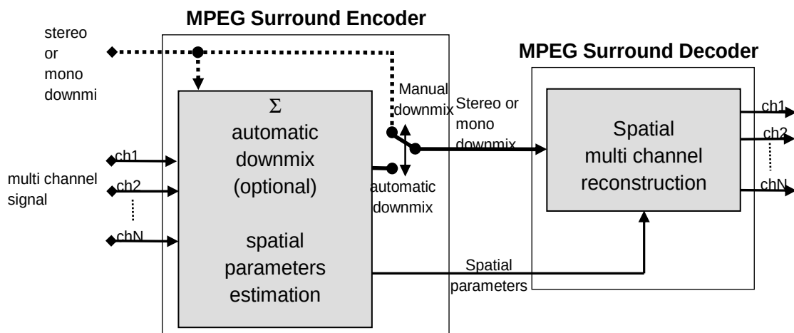
Figure 1a: Principle of MPEG Surround, the downmix is coded using MPEG-1 Layer II
