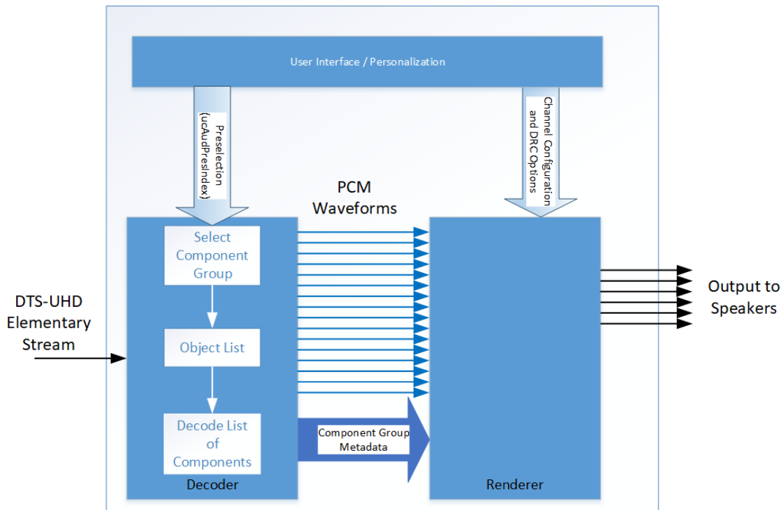
Figure 10: Component Group Selection Decoded and Rendered
