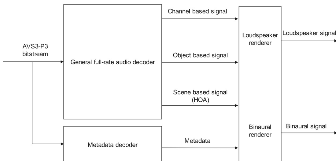
Figure 12: General full-rate audio decoder framework
