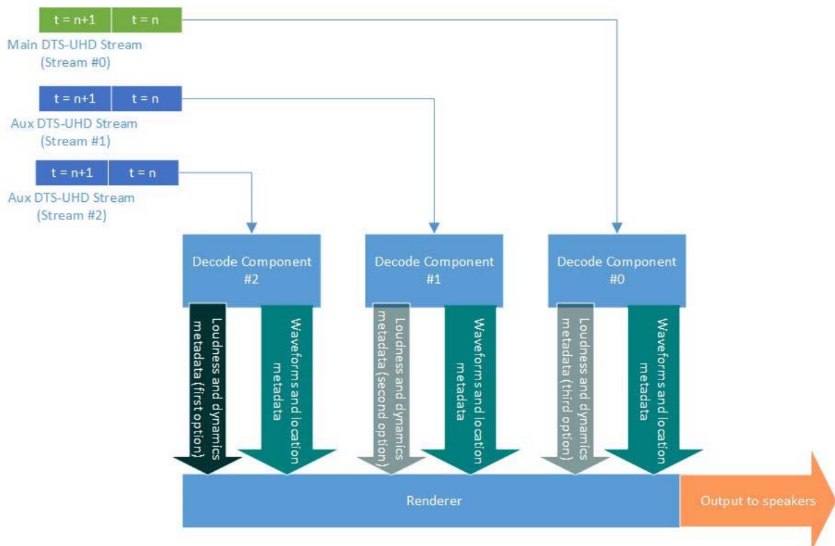
Figure 11: DTS-UHD Multi-stream Example
