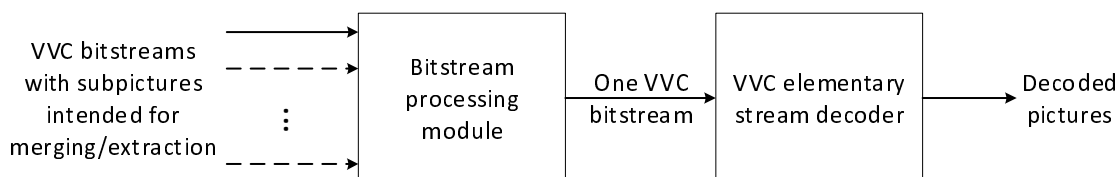
Figure M.2: A bitstream processing module is necessary to take advantage of VVC subpictures
