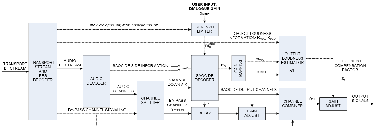
Figure E.7: Loudness compensation in the case of multichannel service with Dialogue Enhancement
