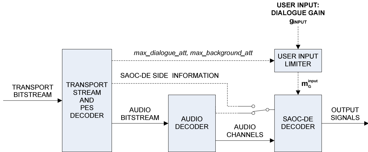
Figure E.5: Stereo service with Dialogue Enhancement
