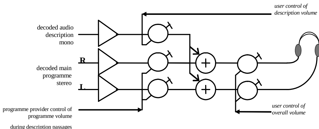
Figure E.1: Functionality of AD decoder processing
