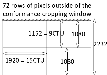
Figure M.4: Usage of the conformance cropping window for a 4K mosaic made of 2x2 HD subpictures
