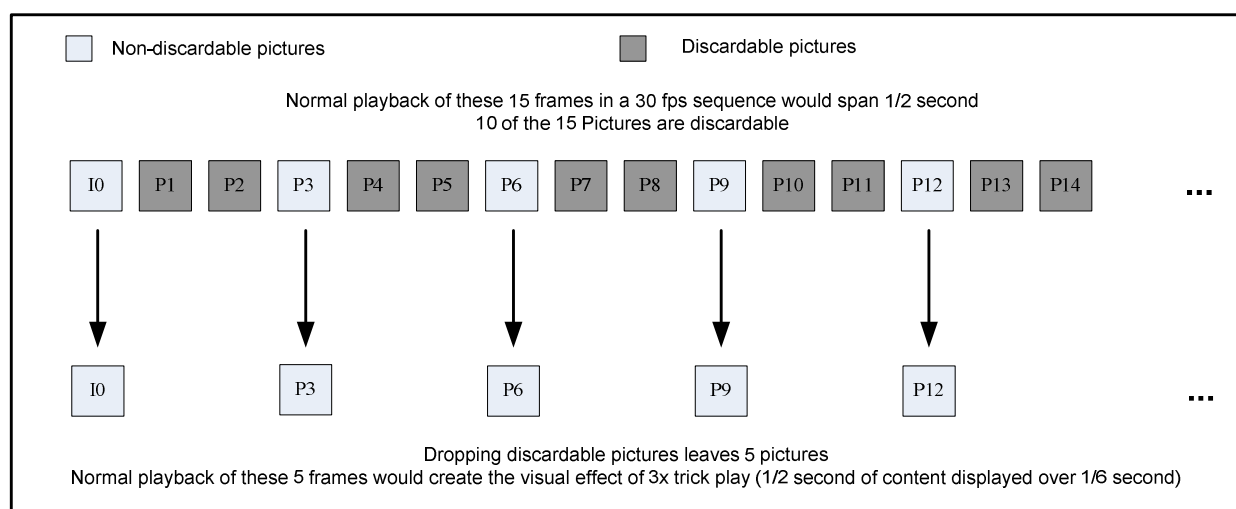
Figure F.3: Coding Structure with 2 Out of Every 3 Pictures as Discardable Pictures (the Discardable Pictures are inserted consistently)
