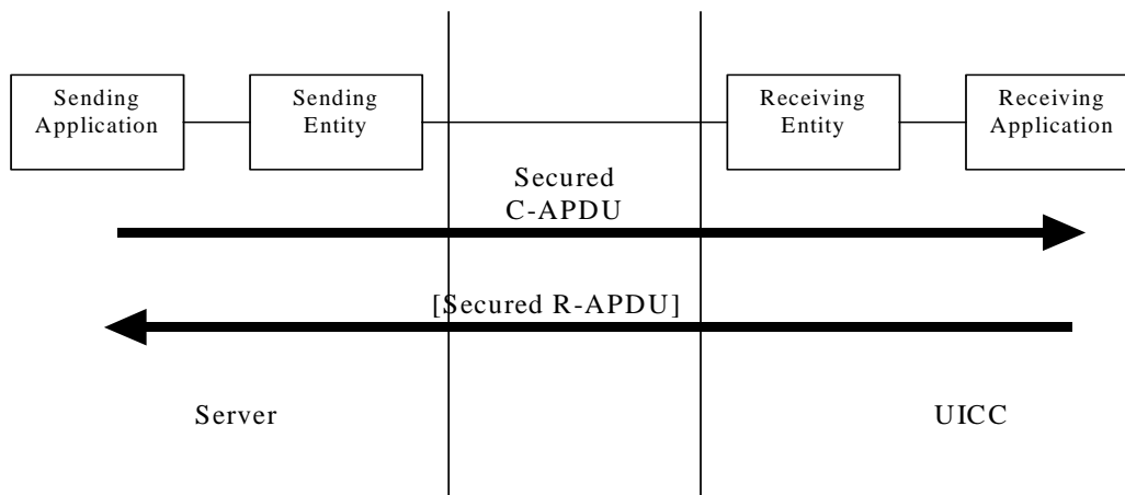
Figure 4.1: Remote management
