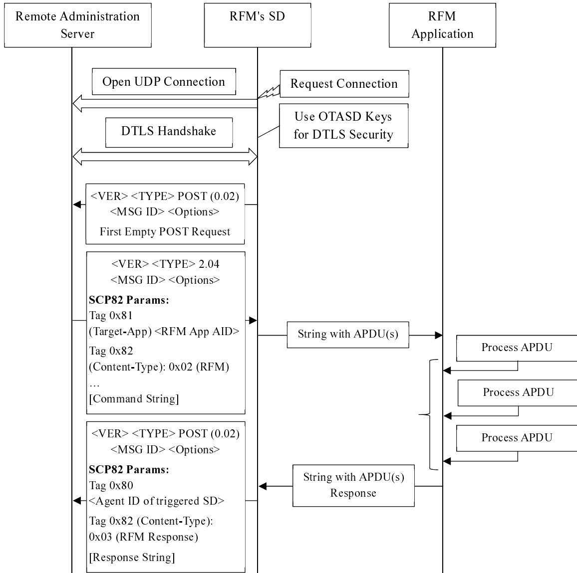
Figure D.1: RFM process communication flow over a DTLS connection
