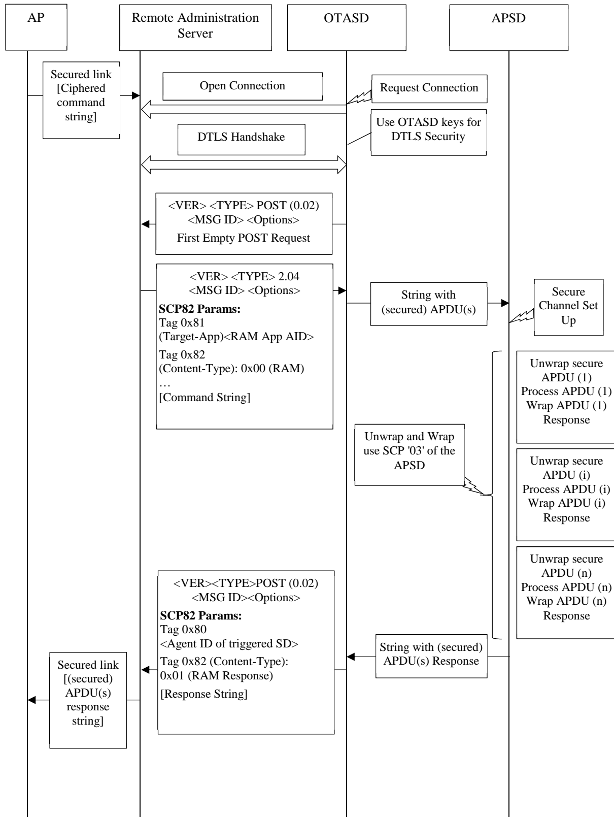
Figure E.2.1: Communication Flow between an AP and its APSD through a Third Party RAS
