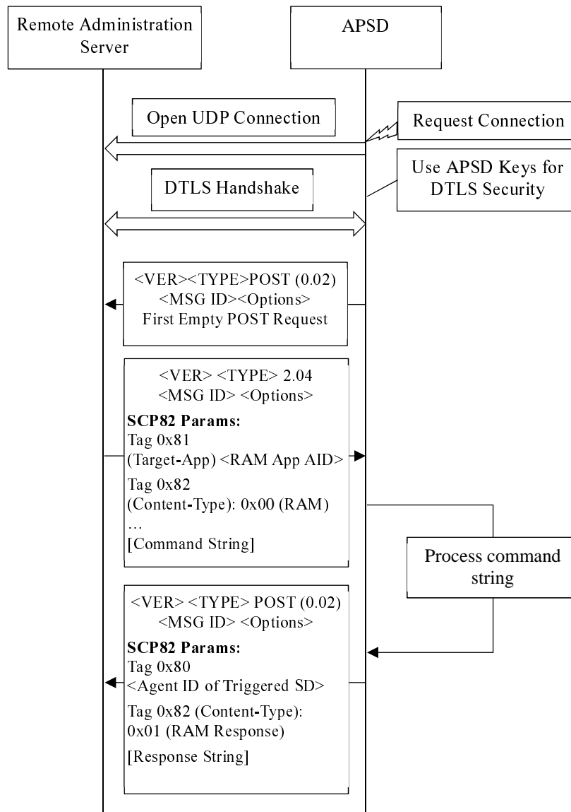
Figure E.1.1: Communication Flow between an AP (Owning a RAS) and its APSD
