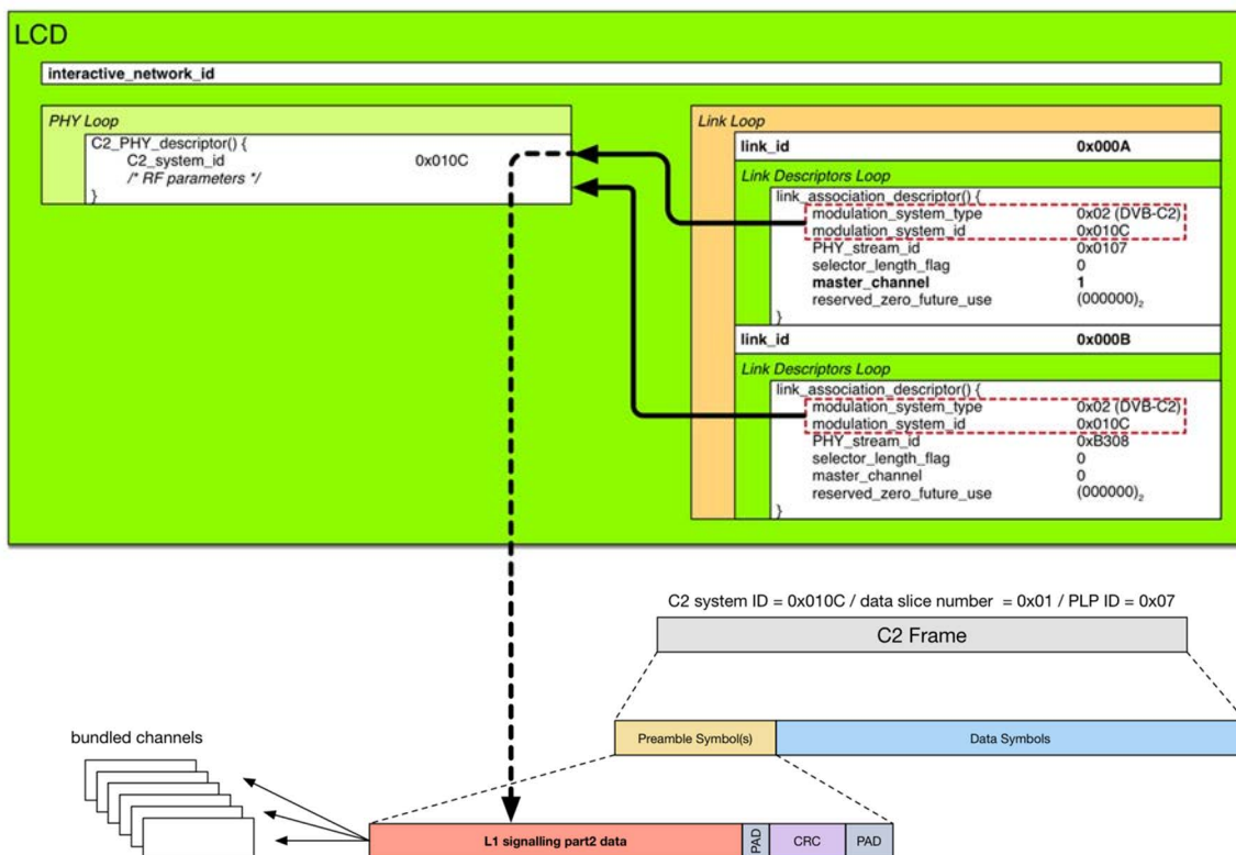
Figure A.6: Example of DVB-C2 channel bundling
