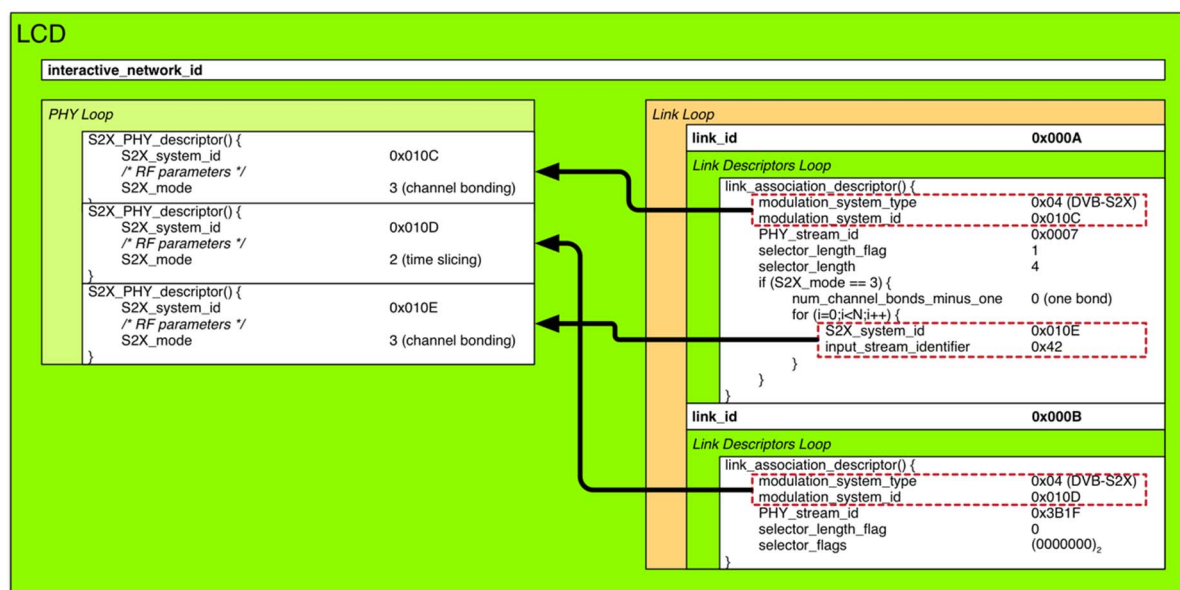
Figure A.7: Example of DVB-S2X channel bonding and time slicing
