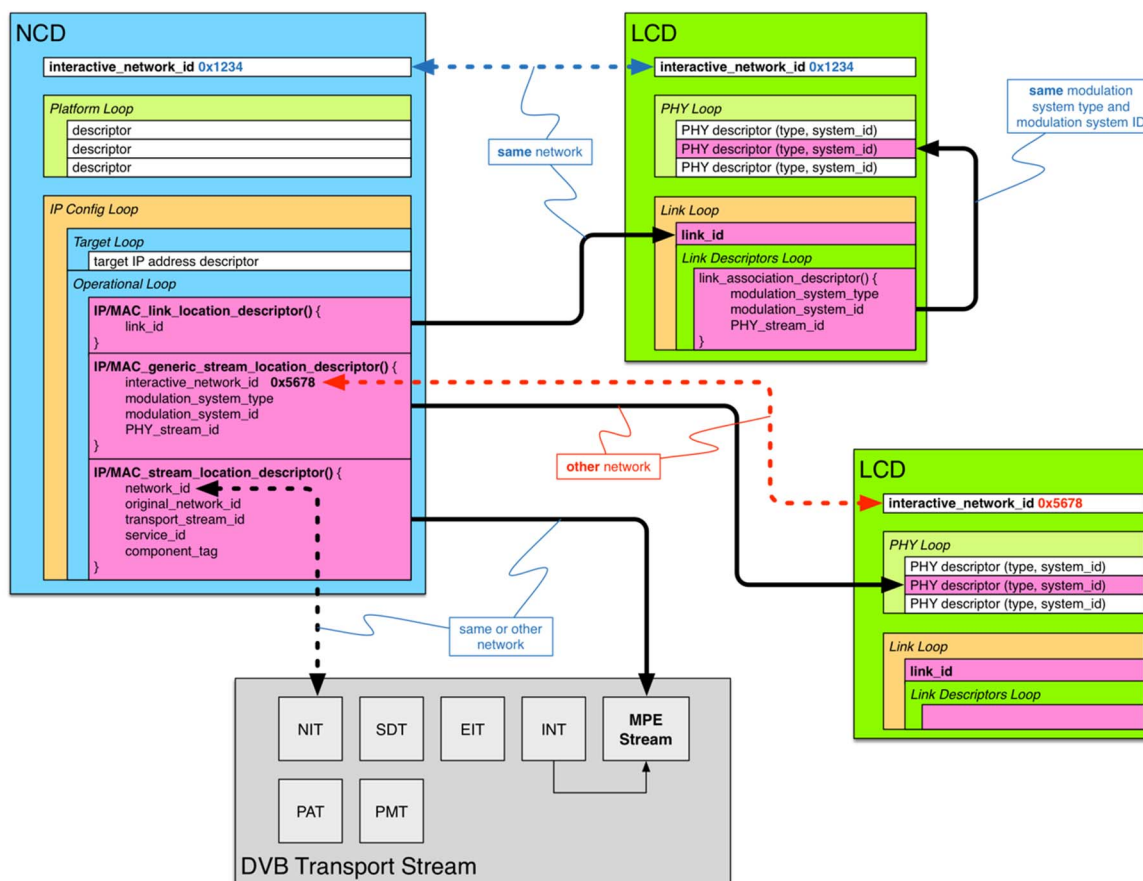
Figure A.4: Mapping to LLC tables across networks, and to Transport Stream resources
