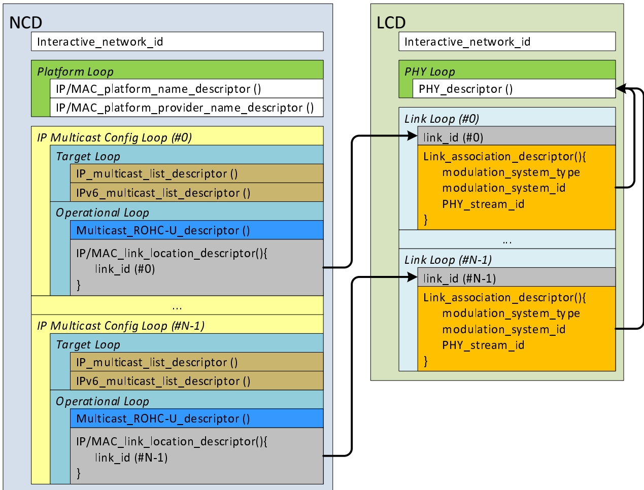
Figure A.8: Example of NCD and LCD for Multicast stream transport in DVB-GSE
