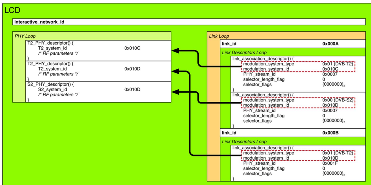
Figure A.5: Example of carriage of Links on different physical layers
