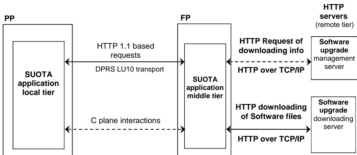
Figure 2: Application scenario for Software Upgrade Over The Air (SUOTA)
