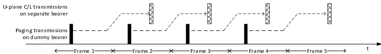
Figure 10: Example of paging burst with U-plane C/L downlink over an additional C/L bearer
