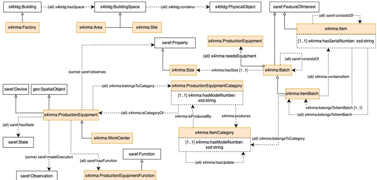
Figure 3: Production Equipment, Factory and related classes
