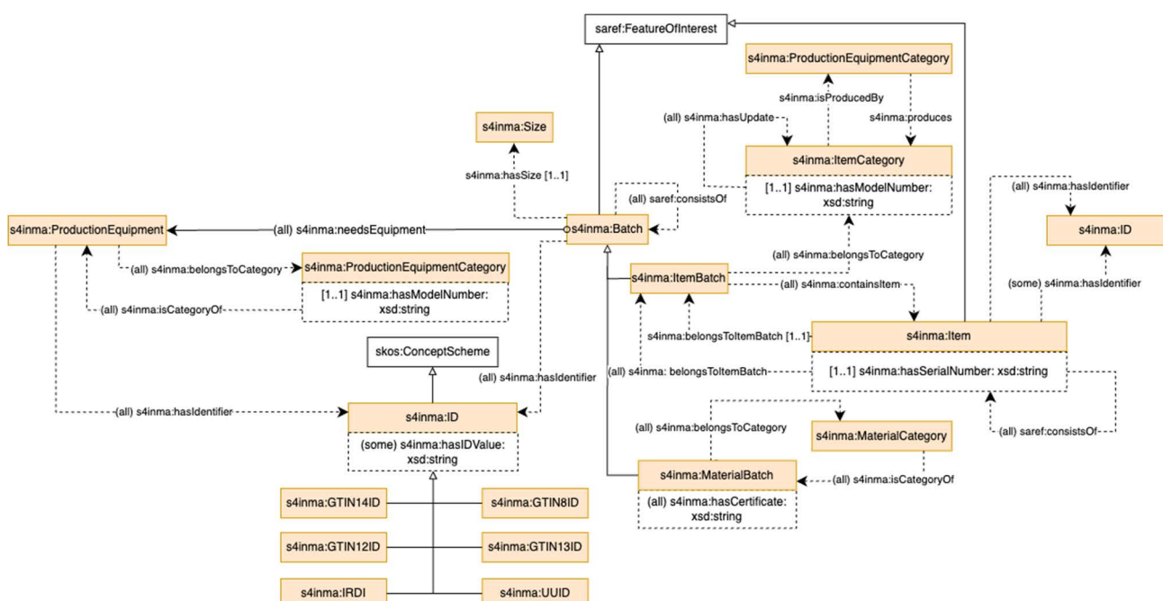
Figure 2: Item, Batch and related classes
