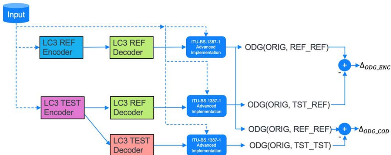
Figure 7.2: \Delta_{ODG} calculation procedure for Encoder and EncDec tests
