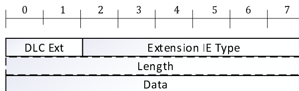
Figure 5.3.3.3-1: DLC Extension Header
