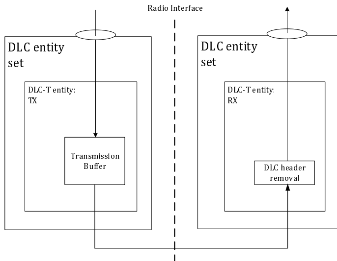
Figure 4.3.1.2-1: DLC Service Type 0 - TX and RX entities
