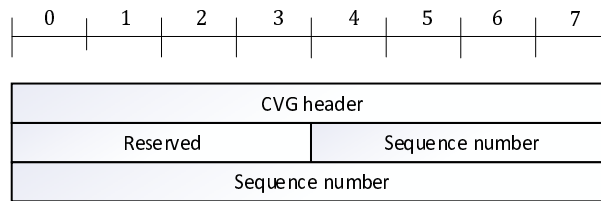
Figure 6.3.10-1: ARQ Poll IE
