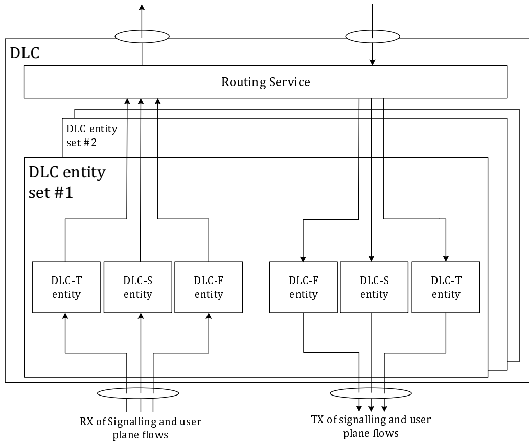
Figure 4.2.2-2: DLC architecture
