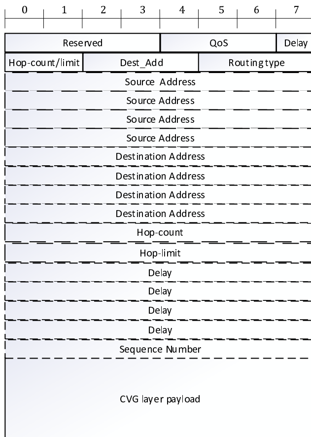
Figure 5.3.4-1: SDU structure for routing
