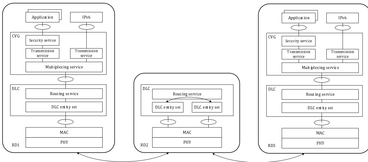
Figure 4.2.1-2: Illustration of the overall protocol architecture for mesh networking
