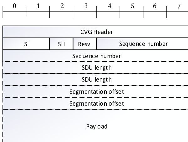
Figure 6.3.4-1: Data IE
