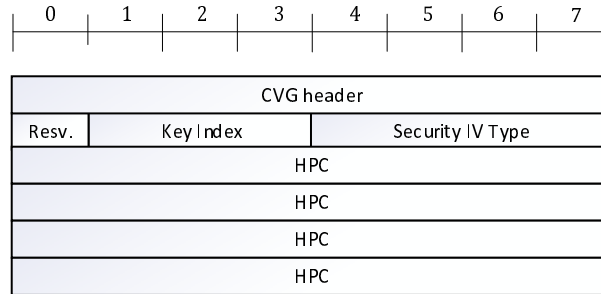
Figure 6.3.7-1: Security IE
