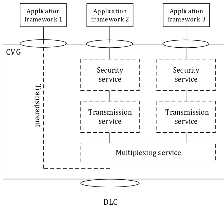
Figure 4.2.3-1: CVG architecture
