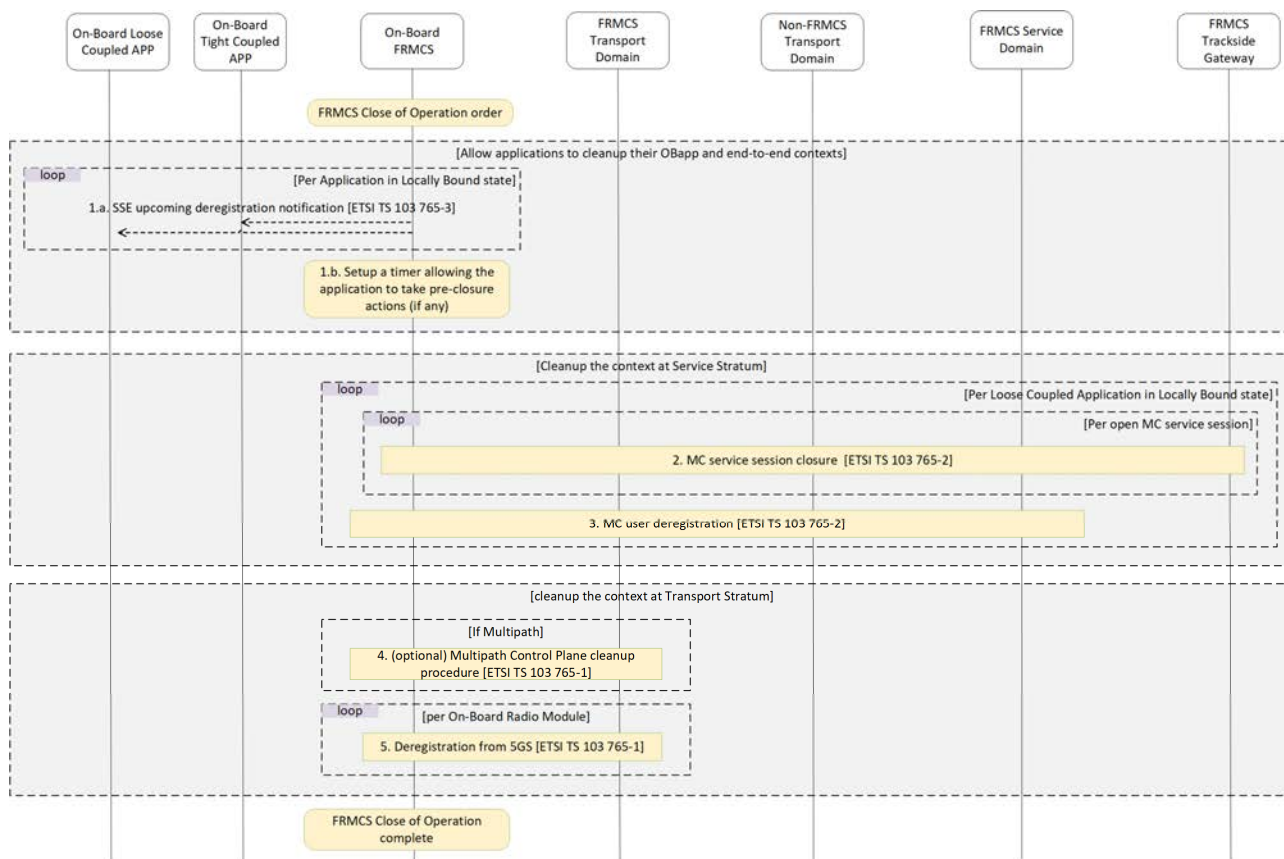
Figure 6.3-1: FRMCS Close of Operation procedure
