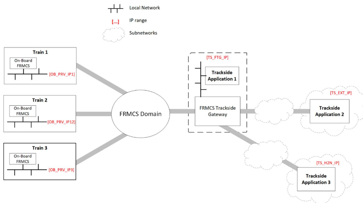
Figure 8.0-1: Variants of IP address H2N ranges of the train networks and of the trackside networks
